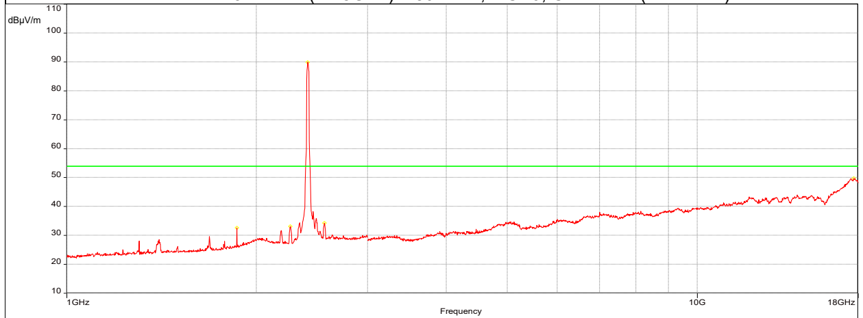
Peak Plot – 3 meters (1-18GHz) – 802.11n, MCS0, Channel 1 (2412MHz)
