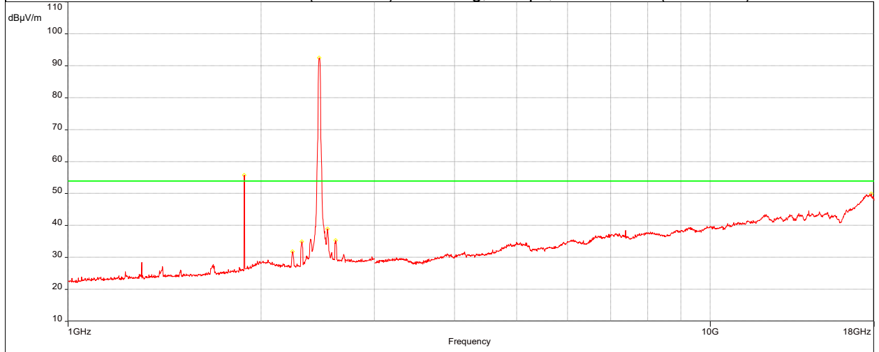
Peak Plot – 3 meters (1-18GHz) – 802.11g, 6Mbps, Channel 11 (2462MHz)
