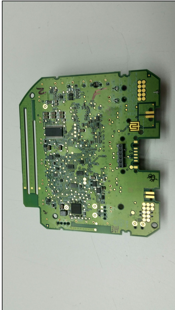
Figure 1: Internal Photo – Front with Shields Removed
