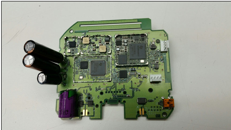
Figure 2: Internal Photo – Back with Shields Removed
