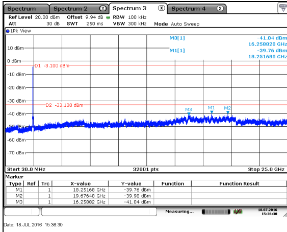
Figure 7.5.1.2-12: 802.11n40 – HCH – 30MHz–25GHz
