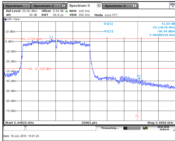
Figure 7.5.1.2-18: 802.11n20 – Upper Band-edge
