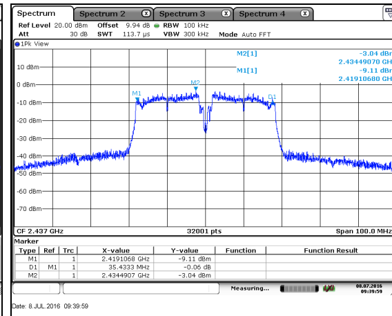
Figure 7.3.2-20: 6dB BW – 802.11n40 – MCH
