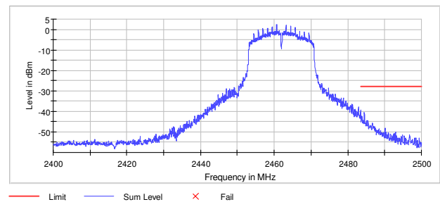
Figure 7.5.1.2-9: 802.11n20 – Upper Band-edge
