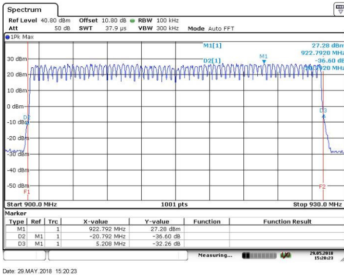
Figure 7.5.1.2-13: Band Edges – OFDM – 200kbps
