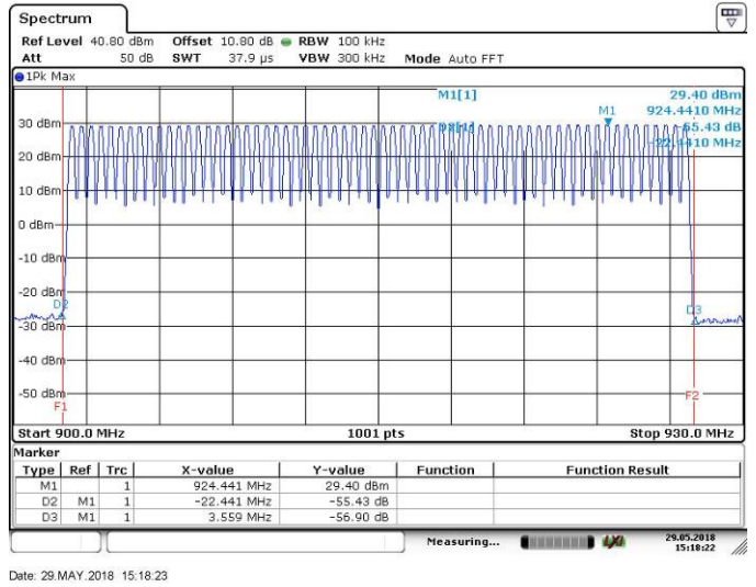
Figure 7.5.1.2-12: Band Edges – FSK – 150kbps
