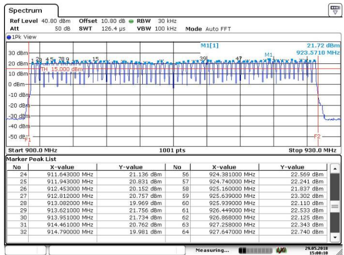
Figure 7.4.2.2-4: No. of Channels – OFDM – 600kbps
