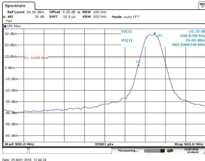
Figure 7.5.1.2-3: Lower Band-edge – FSK – 150kbps
