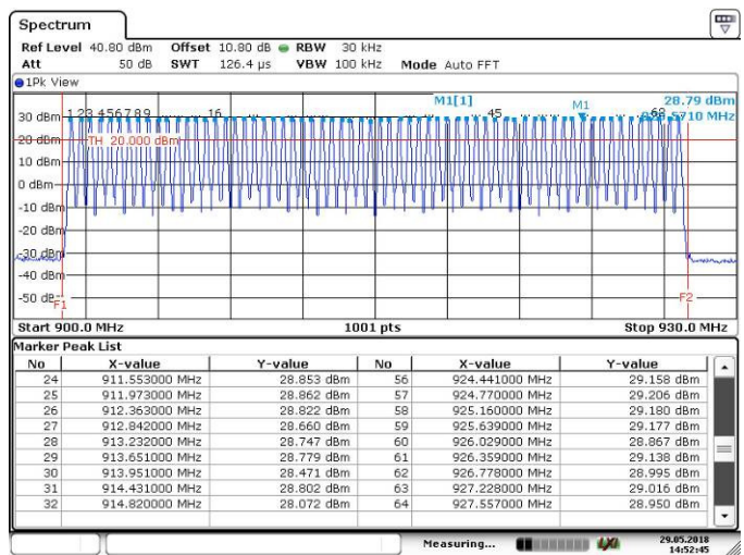
Figure 7.4.2.2-2: No. of Channels – FSK – 150kbps
