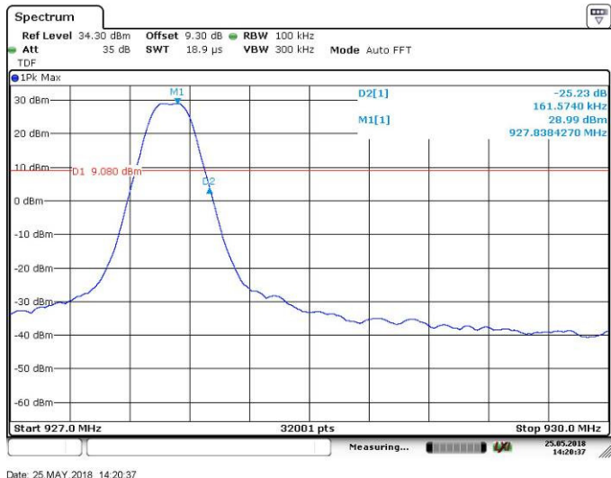
Figure 7.5.1.2-4: Upper Band-edge – FSK – 150kbps
