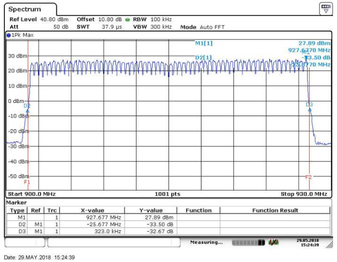
Figure 7.5.1.2-14: Band Edges – OFDM – 600kbps
