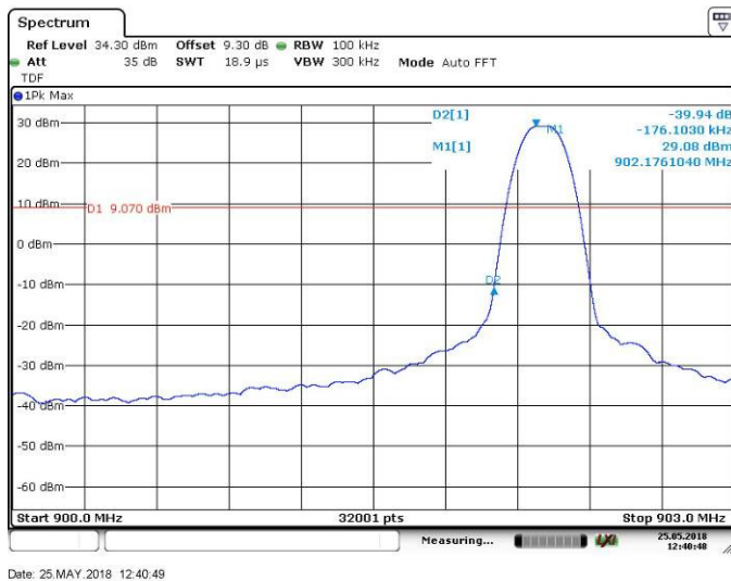
Figure 7.5.1.2-1: Lower Band-edge – FSK – 50kbps
