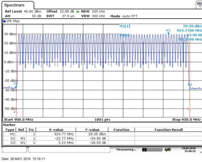
Figure 7.5.1.2-11: Band Edges – FSK – 50kbps
