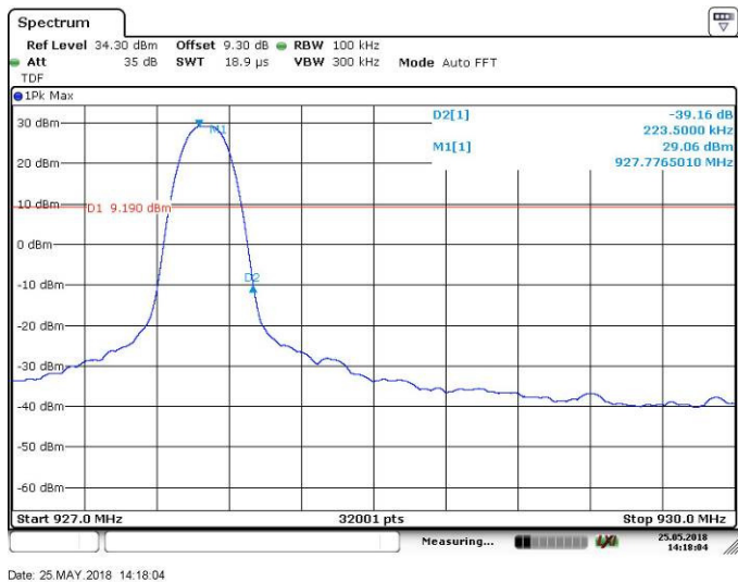
Figure 7.5.1.2-2: Upper Band-edge – FSK – 50kbps
