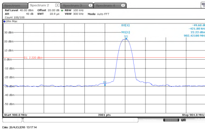
Figure 7.5.1.2-1: Lower Band-edge – FSK – 50kbps
