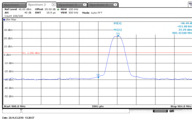
Figure 7.5.1.2-3: Lower Band-edge – FSK – 150kbps
