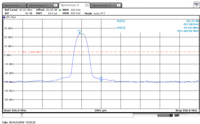
Figure 7.5.1.2-2: Upper Band-edge – FSK – 50kbps
