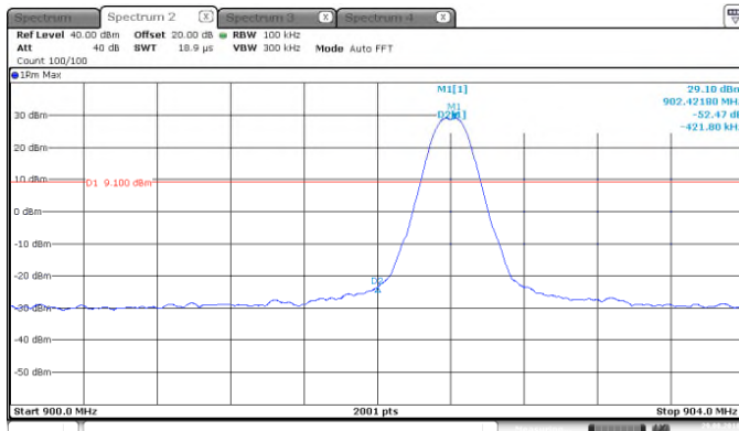
Figure 7.5.1.2-9: Lower Band-edge – DSSS – 12.5kbps
