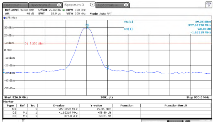
Figure 7.5.1.2-10: Upper Band-edge – DSSS – 12.5kbps
