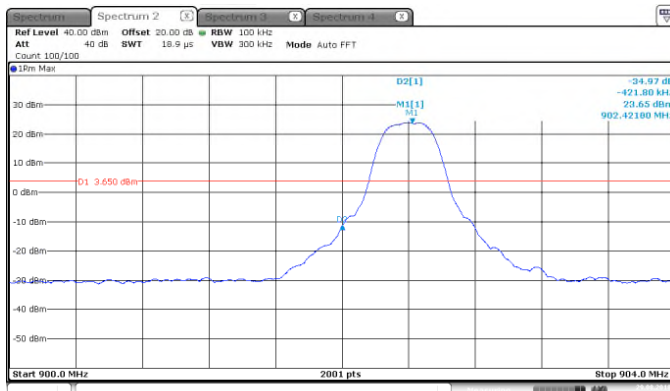
Figure 7.5.1.2-5: Lower Band-edge – OFDM – 200kbps
