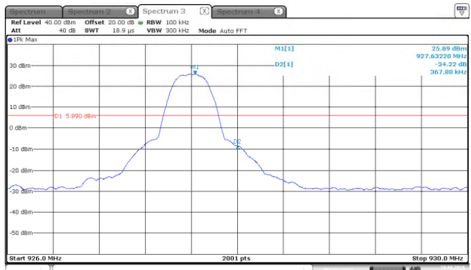
Figure 7.5.1.2-6: Upper Band-edge – OFDM – 200kbps
