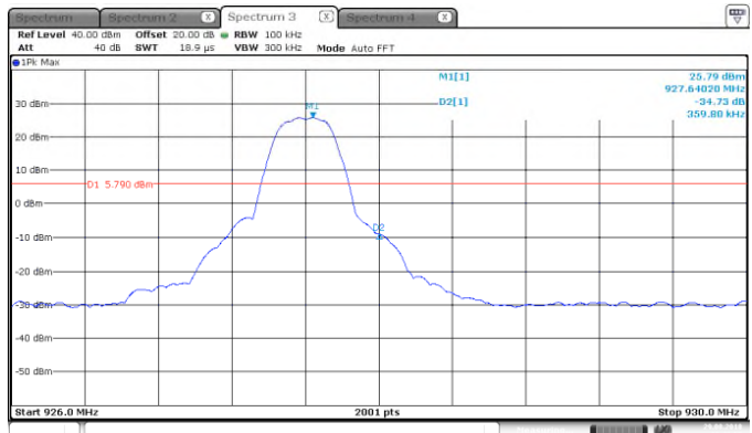
Figure 7.5.1.2-8: Upper Band-edge – OFDM – 600kbps
