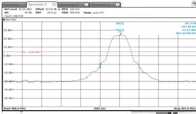
Figure 7.5.1.2-7: Lower Band-edge – OFDM – 600kbps
