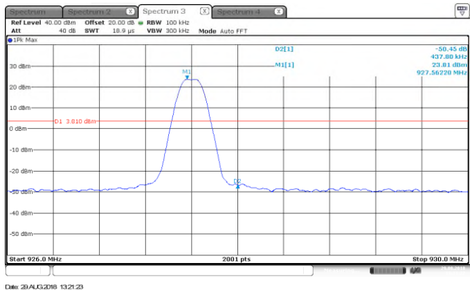
Figure 7.5.1.2-4: Upper Band-edge – FSK – 150kbps
