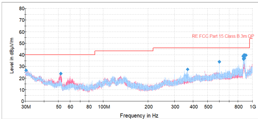
Figure A-3: Reference plot for Radiated Spurious Emissions – 30 MHz – 1 GHz – Whip Antenna
