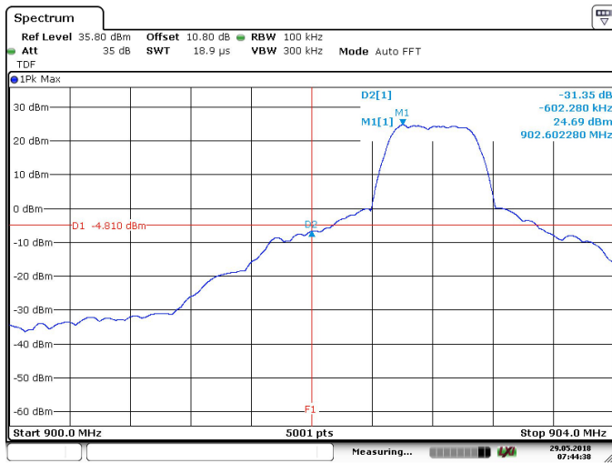
Figure 7.6.1.2-5: Lower Band-edge – No Hopping
