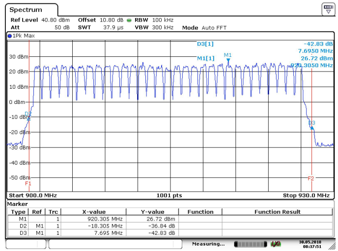
Figure 7.6.1.2-4: Band-edges – Hopping
