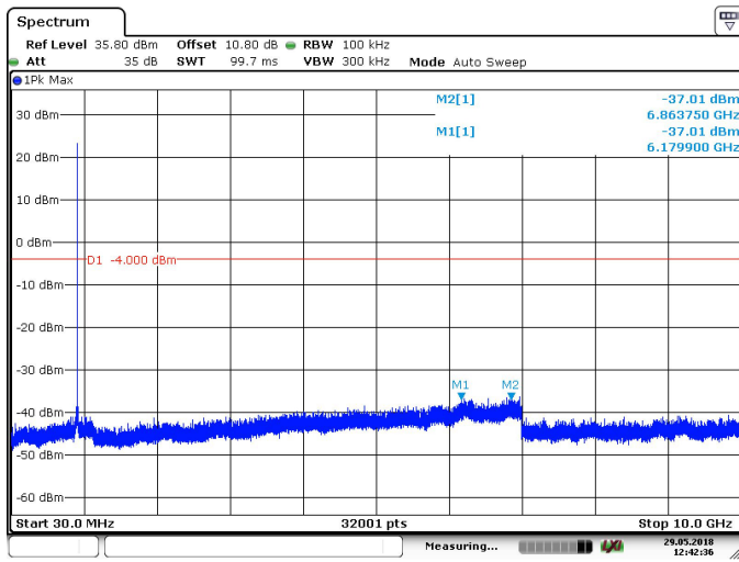
Figure 7.6.1.2-3: 30 MHz – 10 GHz –High Channel
