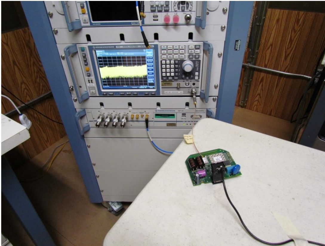
Figure 7: Equipment Under Test – RF Conducted Emissions
