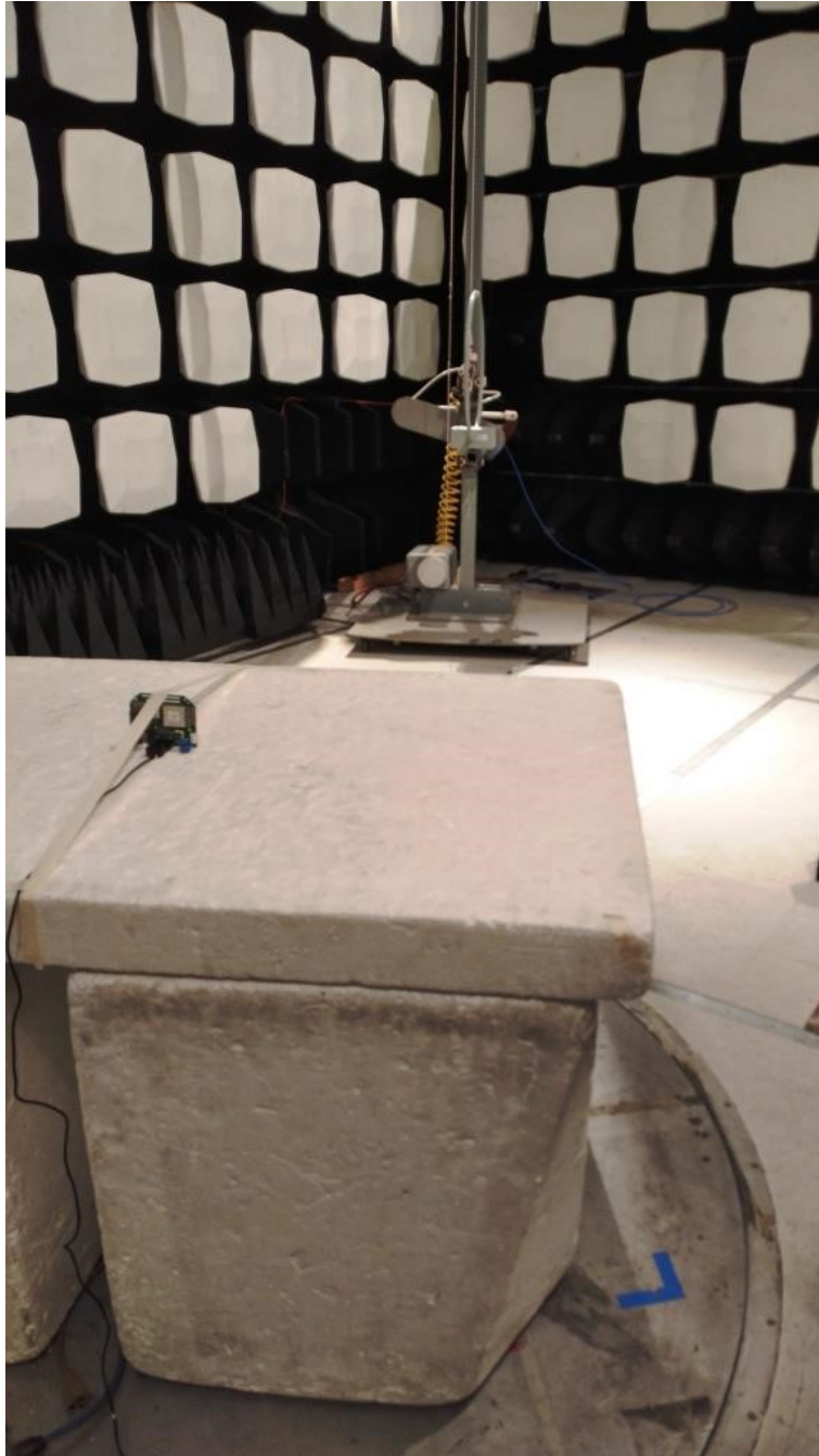
Figure 2: Equipment Under Test – Radiated Emissions – Below 30MHz
