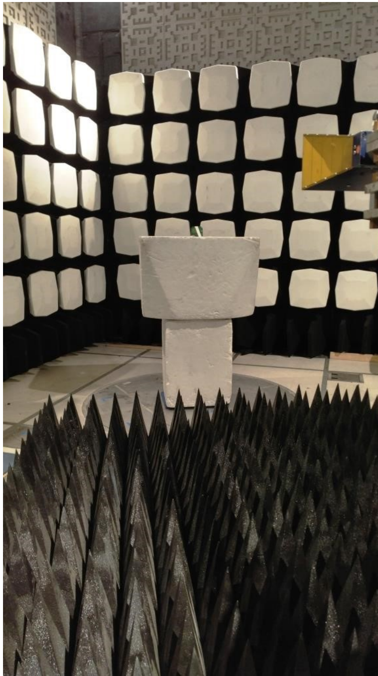
Figure 5: Equipment Under Test – Radiated Emissions – 1-18GHz
