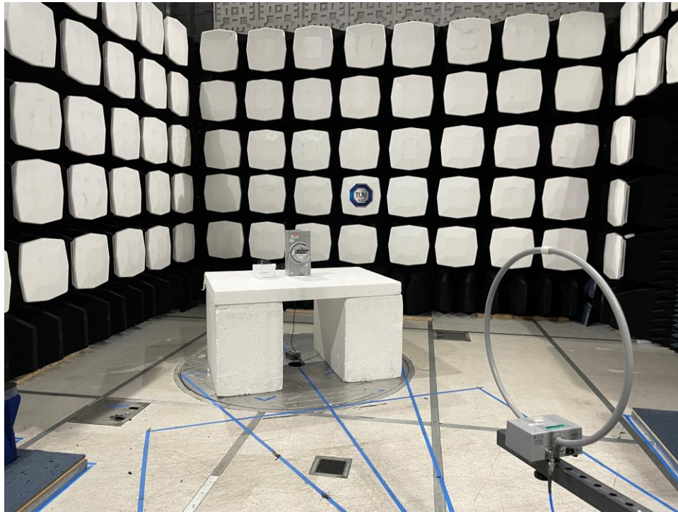
Figure 3: Equipment Under Test – Radiated Emissions <30MHz-Radome antenna
