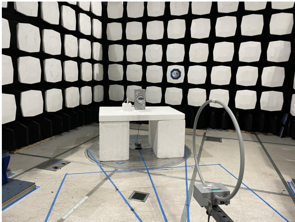
Figure 2: Equipment Under Test – Radiated Emissions <30MHz-Stub antenna
