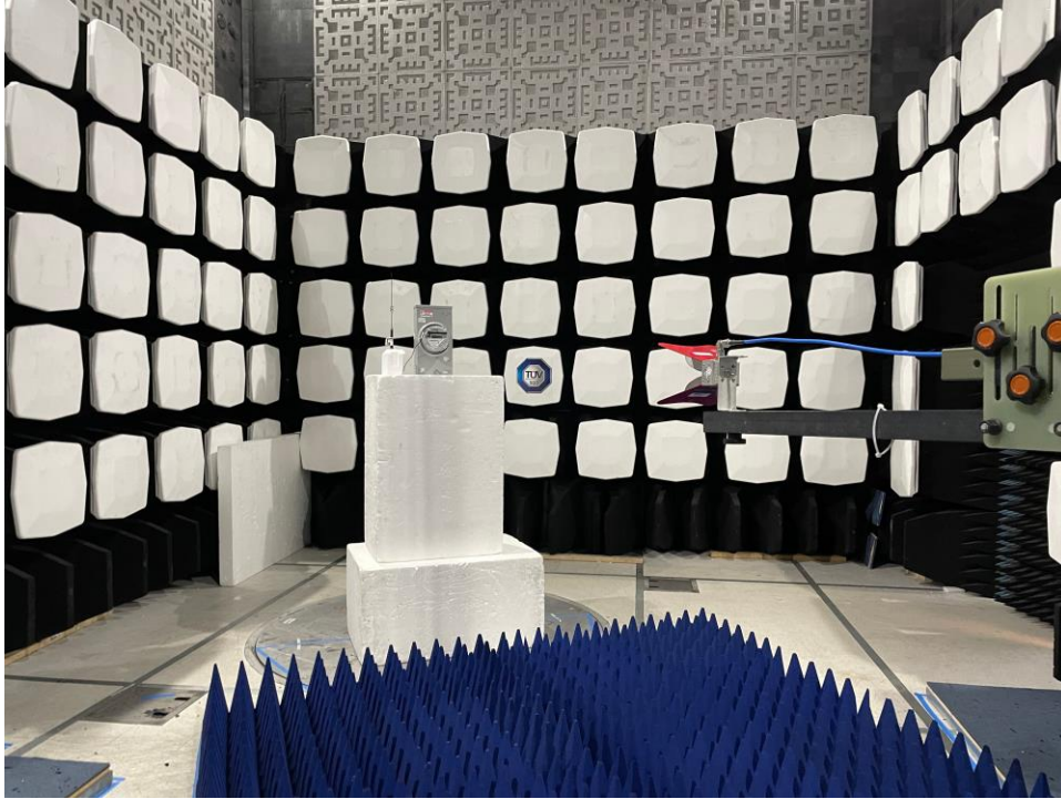
Figure 7: Equipment Under Test – Radiated Emissions >1GHz-Whip Antenna
