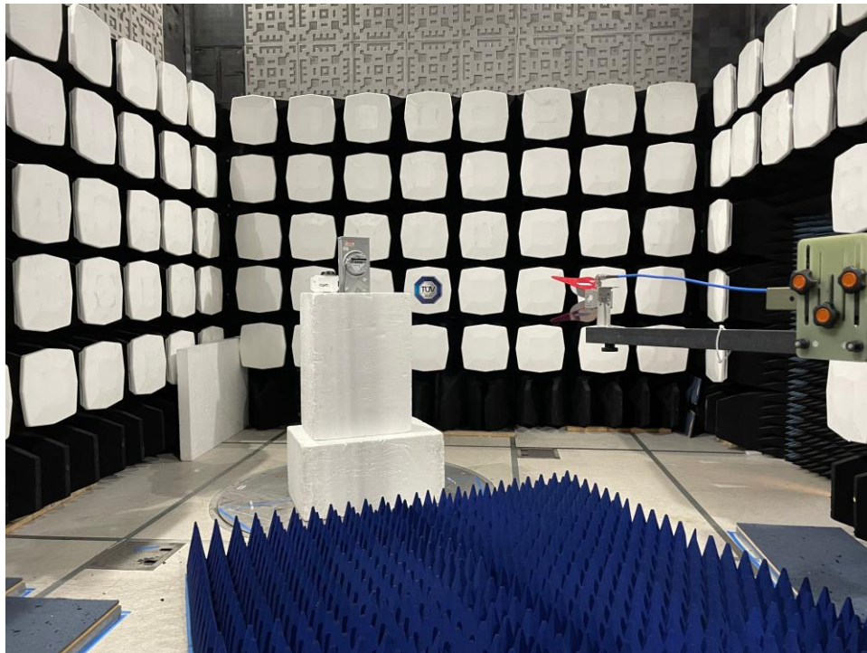
Figure 8: Equipment Under Test – Radiated Emissions >1GHz-Radone Antenna
