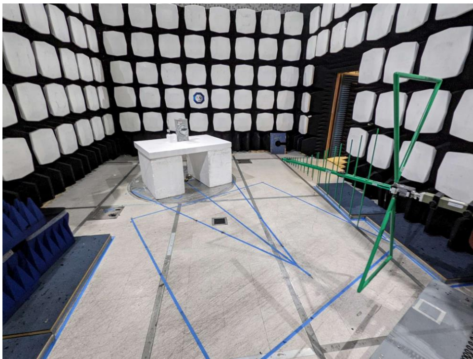
Figure 4: Equipment Under Test – Radiated Emissions <1GHz-Whip Antenna
