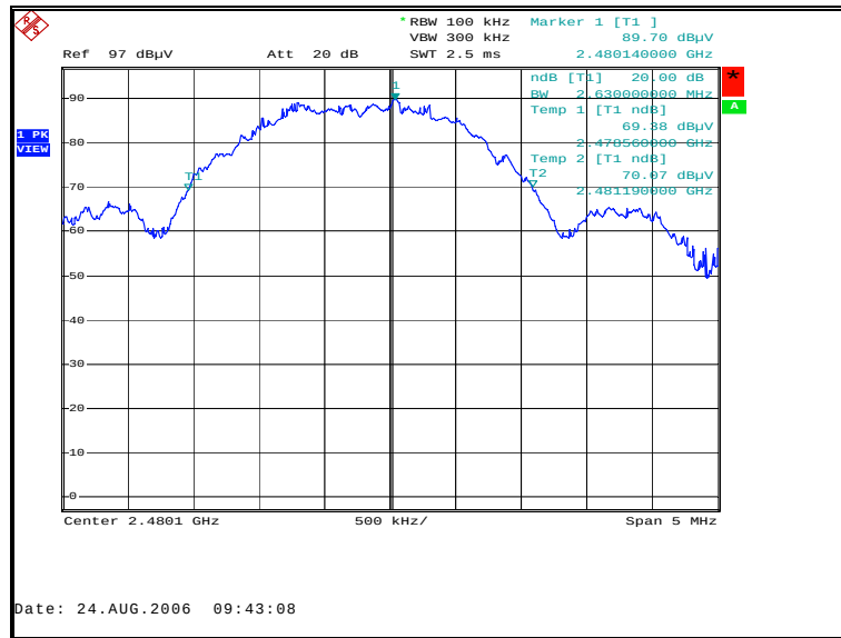
Figure 7.4.2-3 – High Channel
