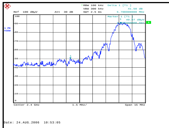
Figure 7.5.1.3-2: Upper Band-edge
