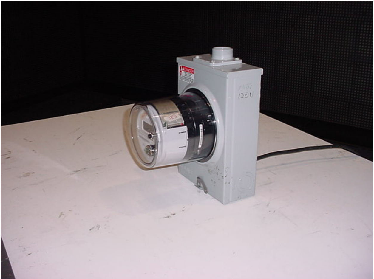
Figure 6: Test Setup – Radiated Emissions – Intentional
