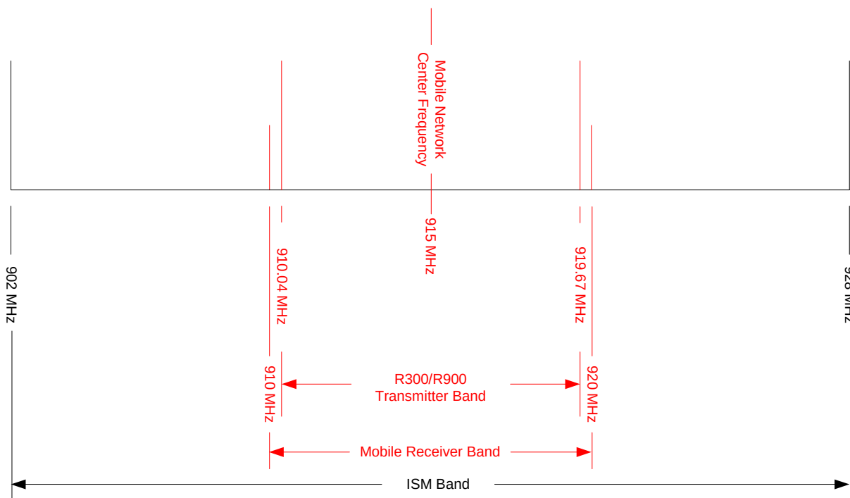
Figure 14 Mobile Network Transmission Bandwidth
