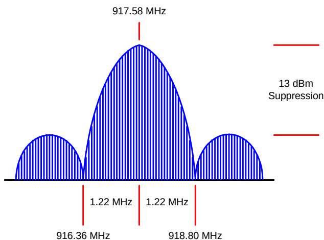
Figure 13 Fixed Network DSSS Pattern
