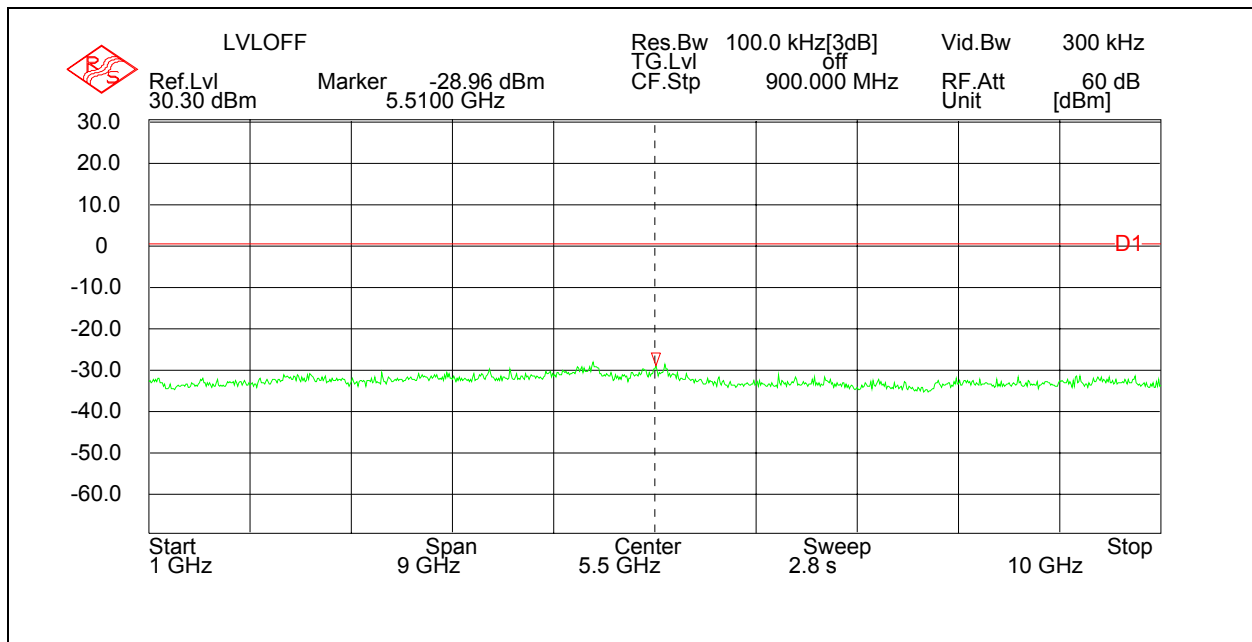
Figure 7.6.2-4 RF Conducted Spurious Emissions – Mid Channel
