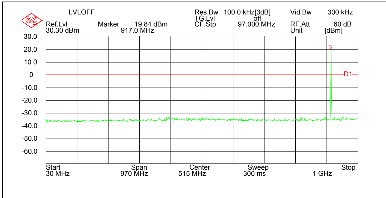
Figure 7.6.2-3 RF Conducted Spurious Emissions – Mid Channel
