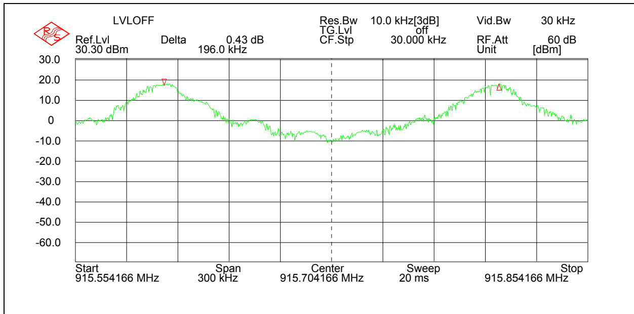
Figure 7.5.1-1: Carrier Frequency Separation
