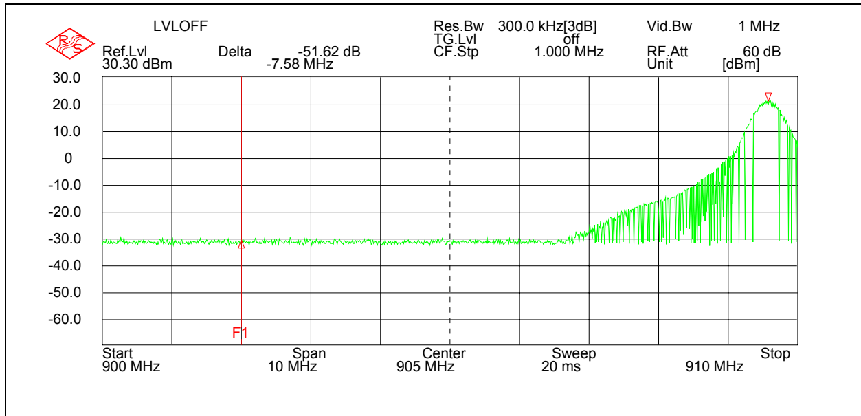
Figure 7.6.1-1: Lower Band-edge
