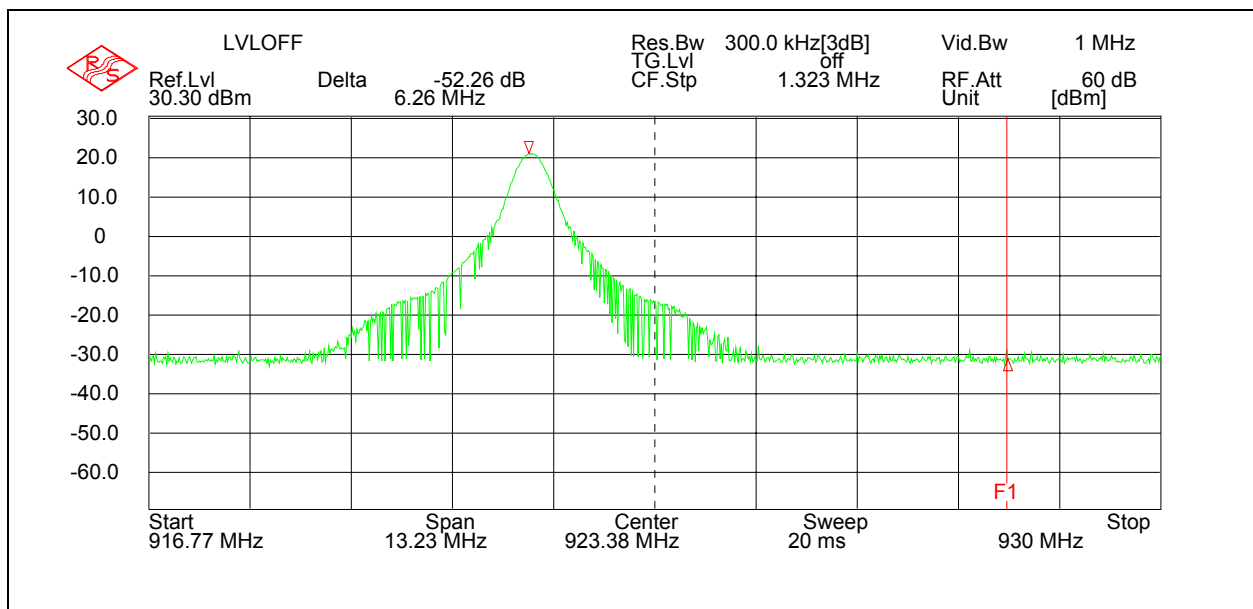
Figure 7.6.1-2: Upper Band-edge
