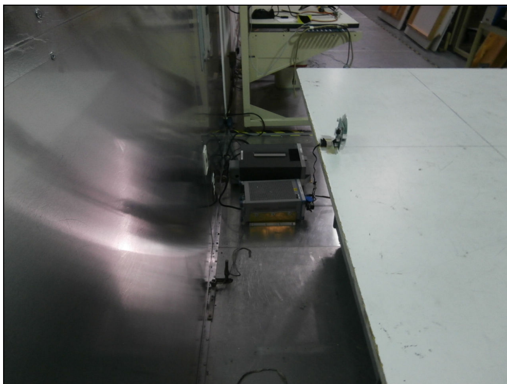
Figure 9: Conducted Emissions
