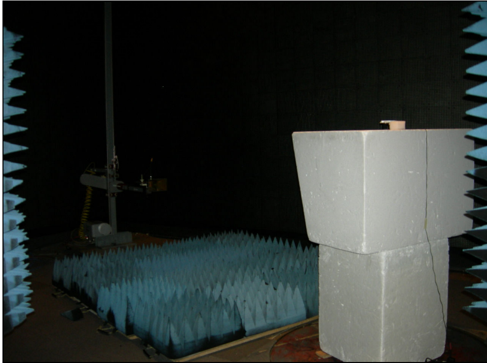
Figure 1: Radiated Emissions
