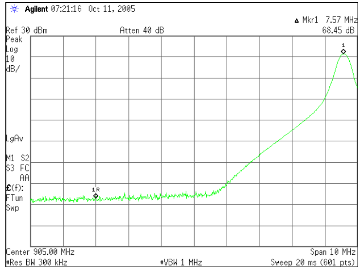
Figure 7.6.1-1: Lower Band-edge
