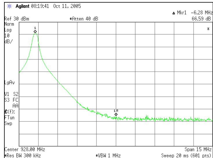
Figure 7.6.1-2: Upper Band-edge
