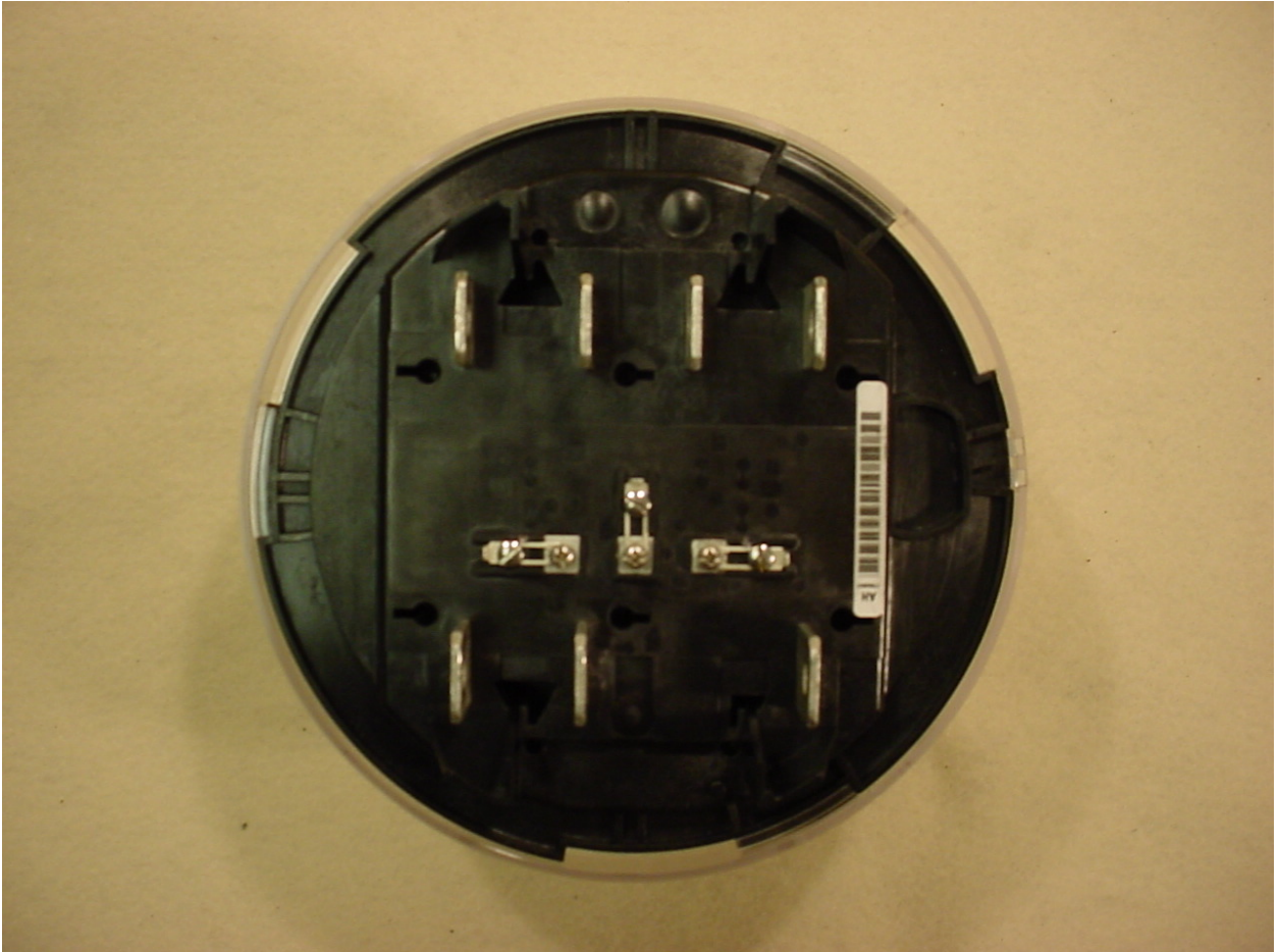
Figure 6: External – Bottom View – Polyphase Metrology Base
