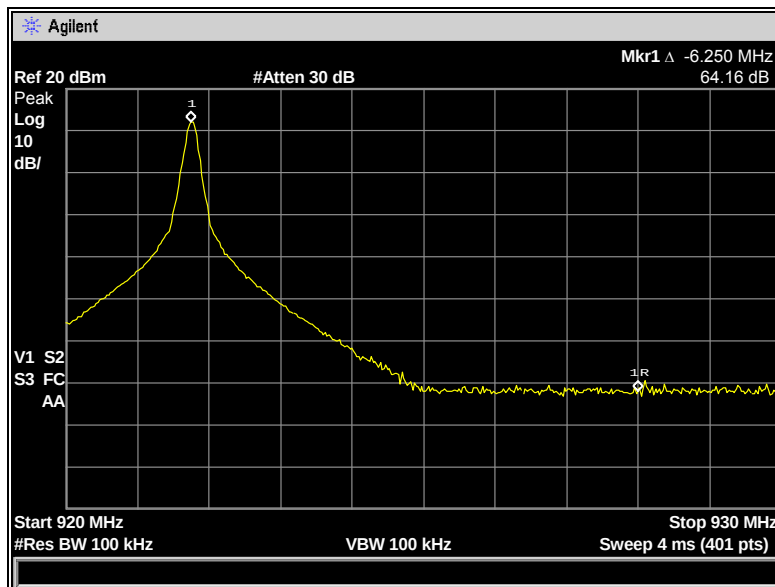
Figure 7.6.1-2: Upper Band-edge
