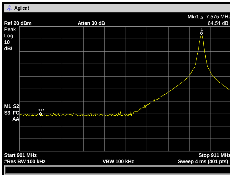
Figure 7.6.1-1: Lower Band-edge
