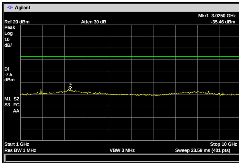
Figure 7.6.2-4 RF Conducted Spurious Emissions – Mid Channel
