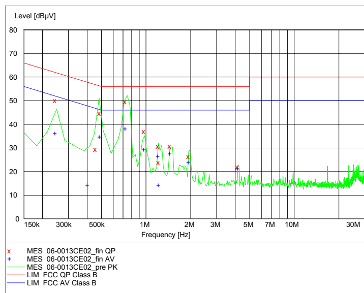
Figure 7.2-2: Conducted Emissions Graph – Line 2
