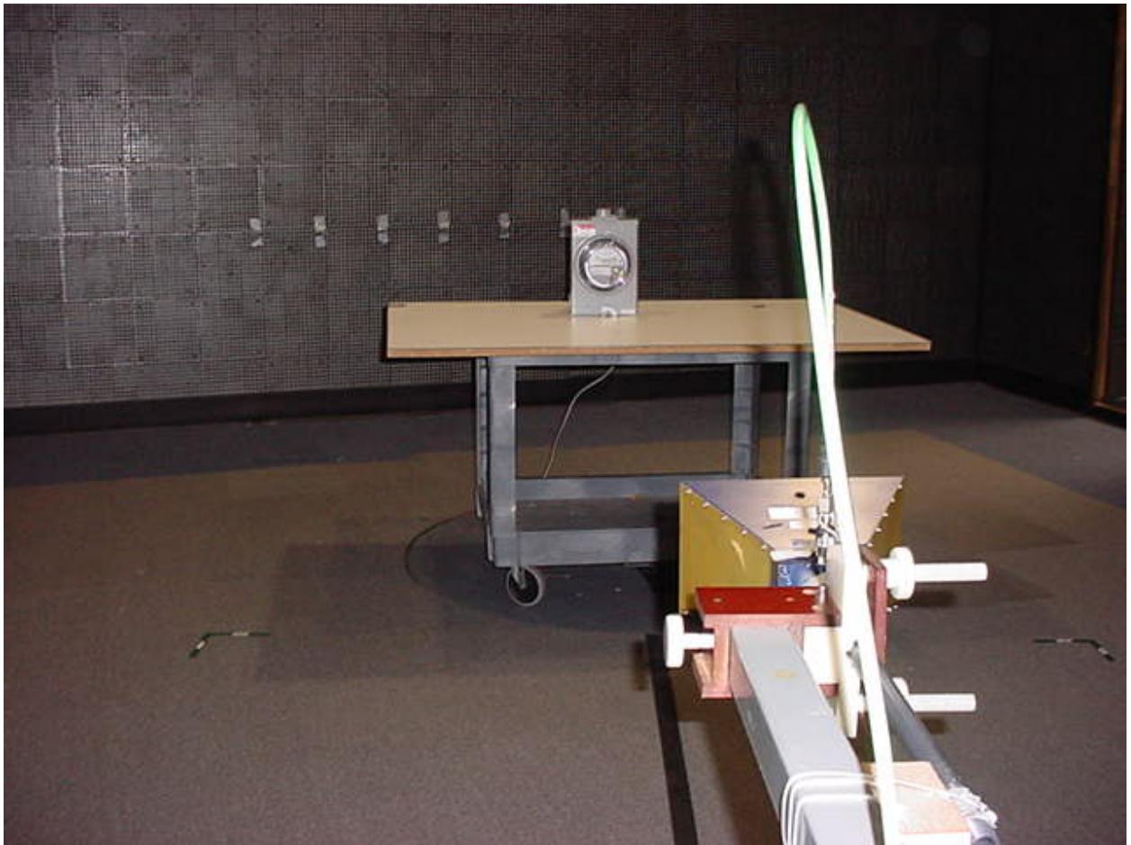
Figure 1: Test Setup – Radiated Emissions - Monophase
