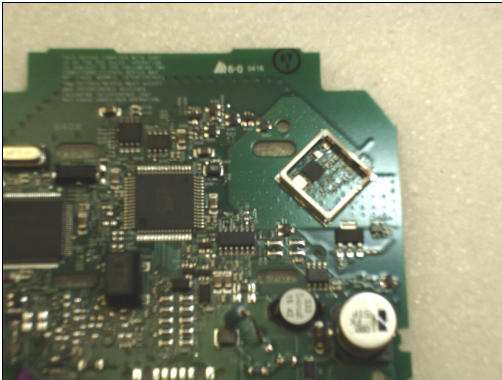
Figure 1: Internal Photo – Without Shield
