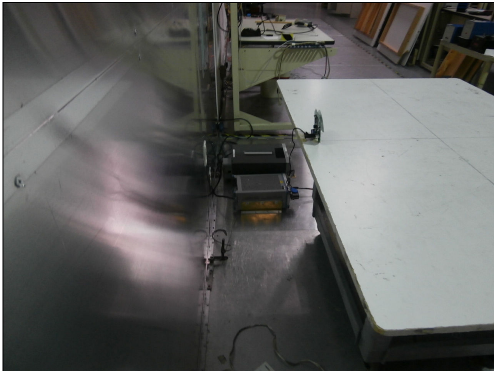
Figure 9: Conducted Emissions
