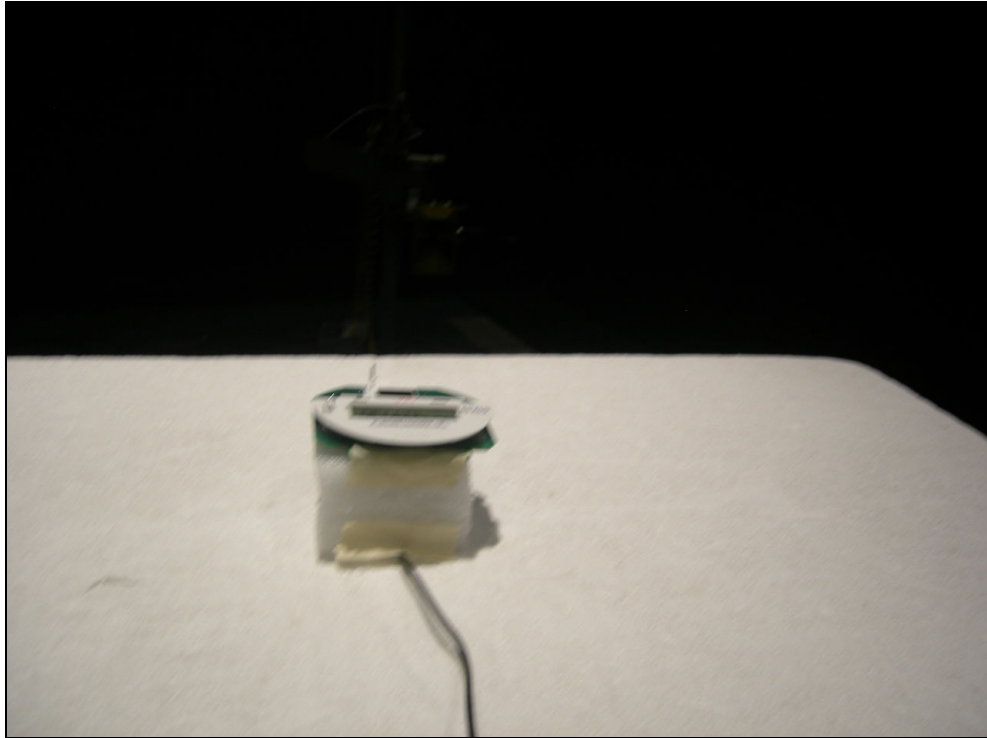
Figure 3: Radiated Emissions – XPOS
