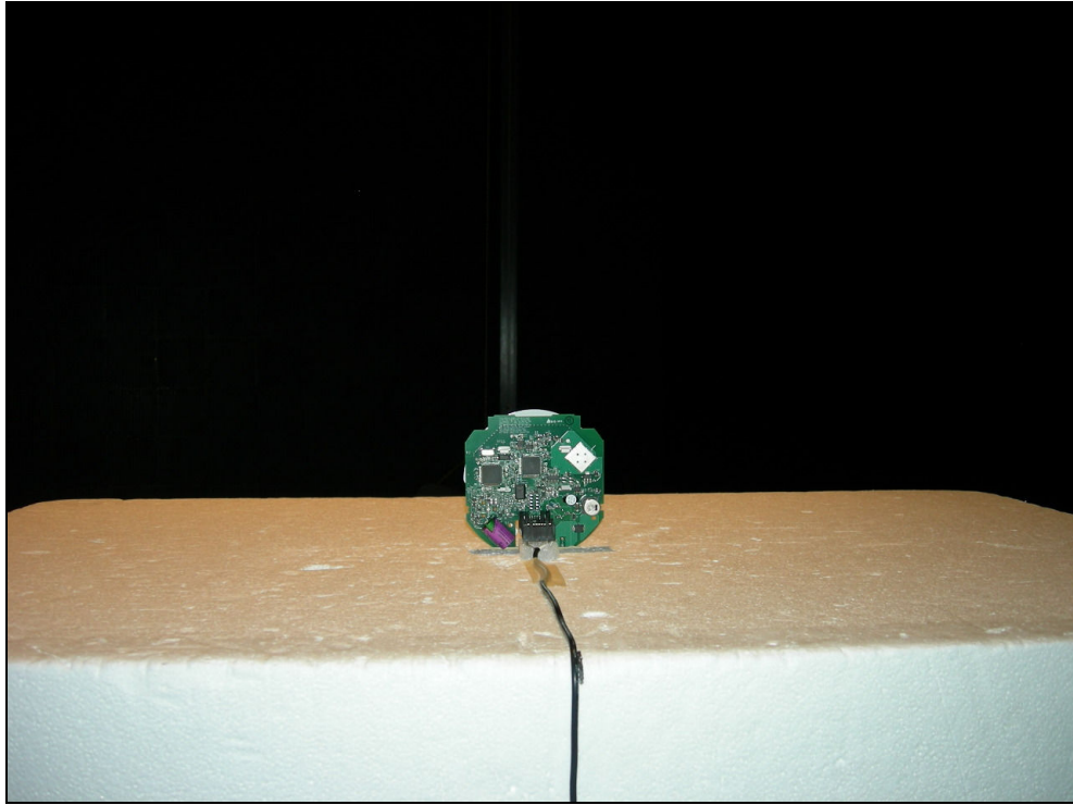
Figure 5: Radiated Emissions – YPOS
