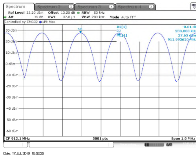
Figure 7.4.1.2-1: Freq. Separation
