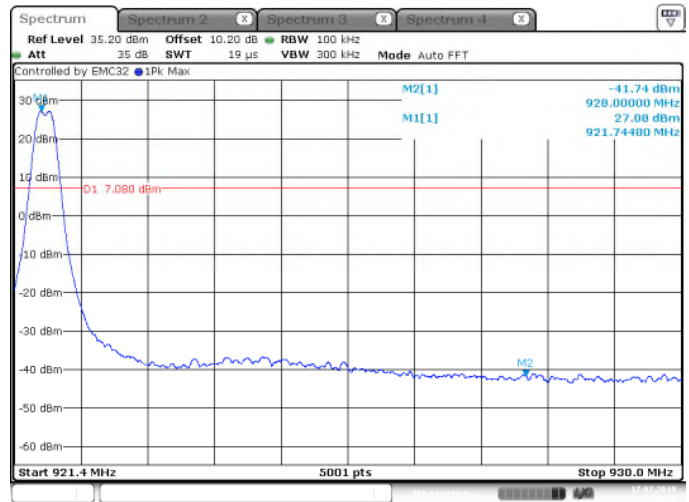
Figure 7.5.1.2-2: Upper Band-edge
