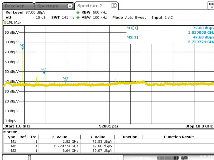
Figure A-4: 1GHz-10GHz
