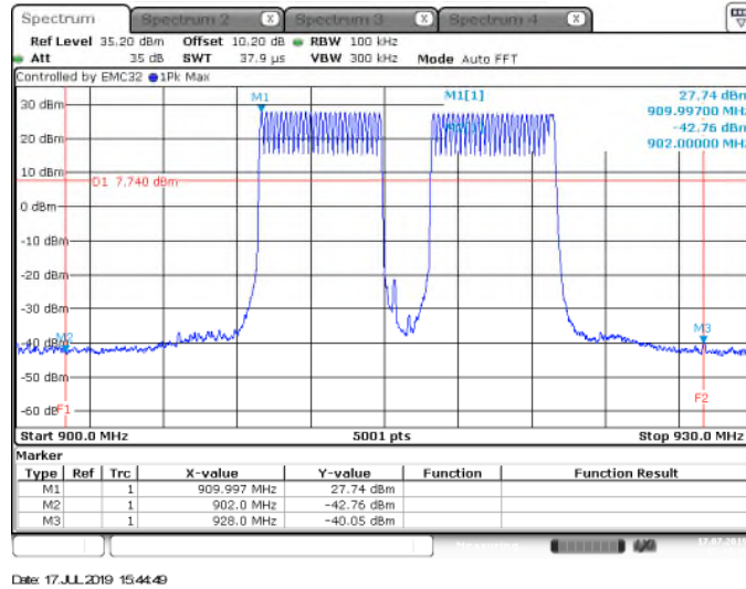
Figure 7.5.1.2-3: Band Edges
