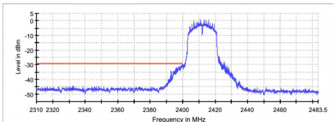
Figure 7.5.1.2-8: 802.11n20 – Lower Band-edge
