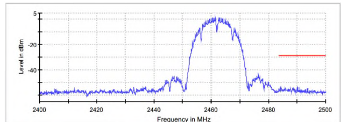
Figure 7.5.1.2-5: 802.11b – Upper Band-edge
