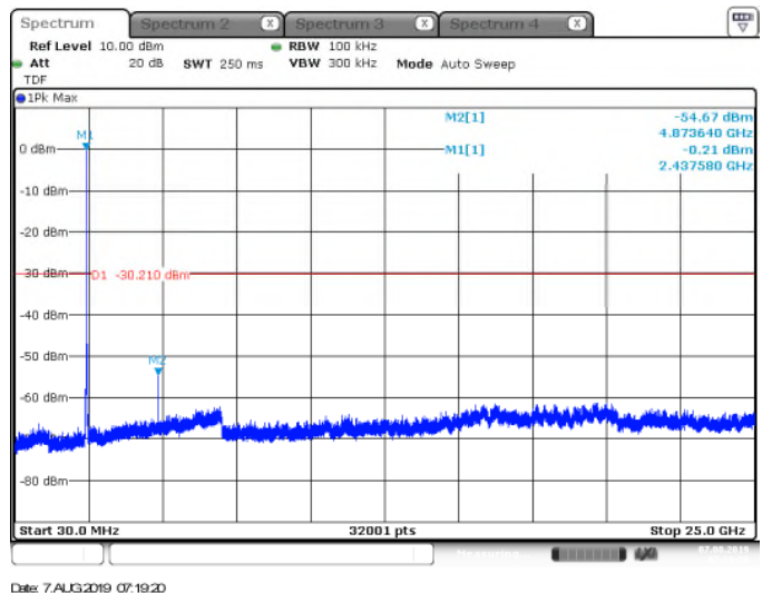
Figure 7.5.1.2-2: 802.11b – MCH – 30MHz–25GHz
