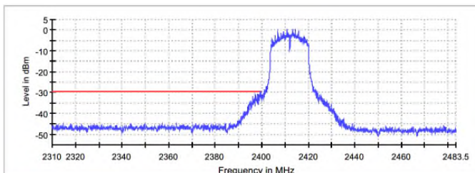
Figure 7.5.1.2-6: 802.11g – Lower Band-edge
