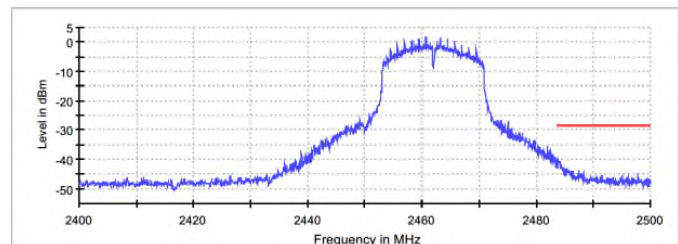
Figure 7.5.1.2-9: 802.11n20 – Upper Band-edge
