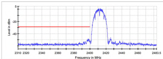
Figure 7.5.1.2-4: 802.11b – Lower Band-edge
