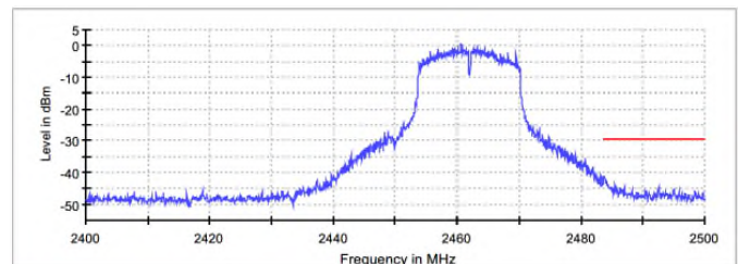
Figure 7.5.1.2-7: 802.11g – Upper Band-edge
