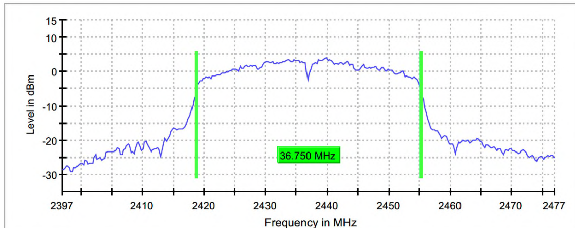
Figure 7.3.2-2: Sample Plot - 99% OBW
