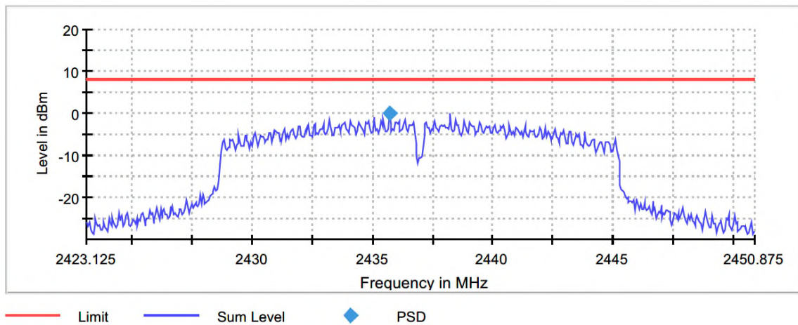
Figure 7.6.2-1: Sample PSD Plot
