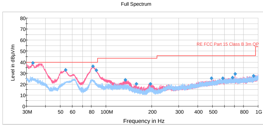
Figure A-3: 30MHz-1GHz
