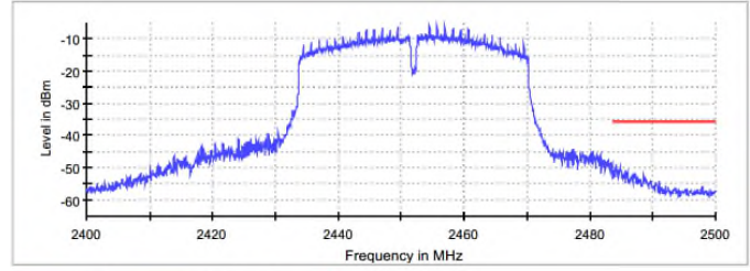
Figure 7.5.1.2-11: 802.11n40 – Upper Band-edge
