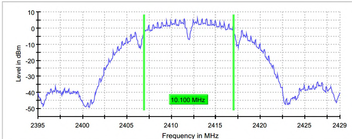
Figure 7.3.2-1: Sample Plot - 6dB BW
