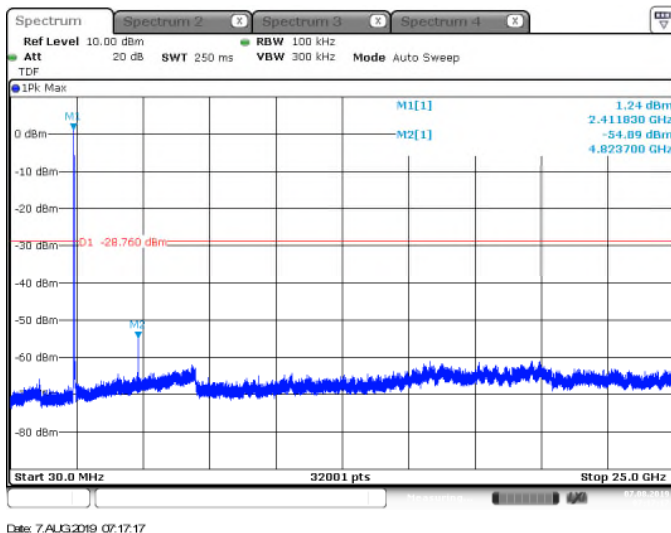
Figure 7.5.1.2-1: 802.11b – LCH – 30MHz–25GHz
