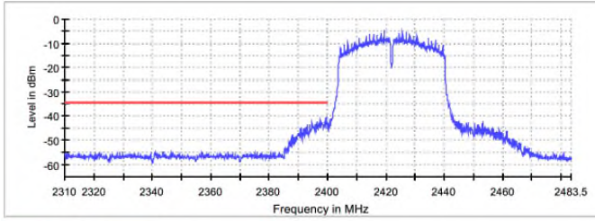
Figure 7.5.1.2-10: 802.11n40 – Lower Band-edge
