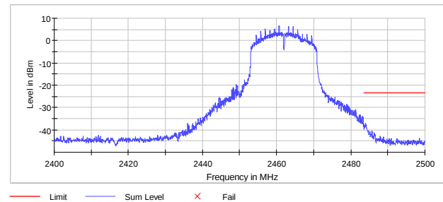
Figure 7.5.1.2-9: 802.11n20 – Upper Band-edge
