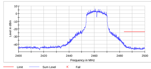
Figure 7.5.1.2-7: 802.11g – Upper Band-edge
