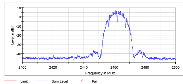
Figure 7.5.1.2-5: 802.11b – Upper Band-edge
