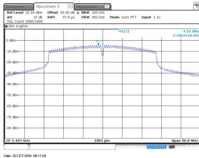
Figure 7.6.2-1: Sample PSD Plot
