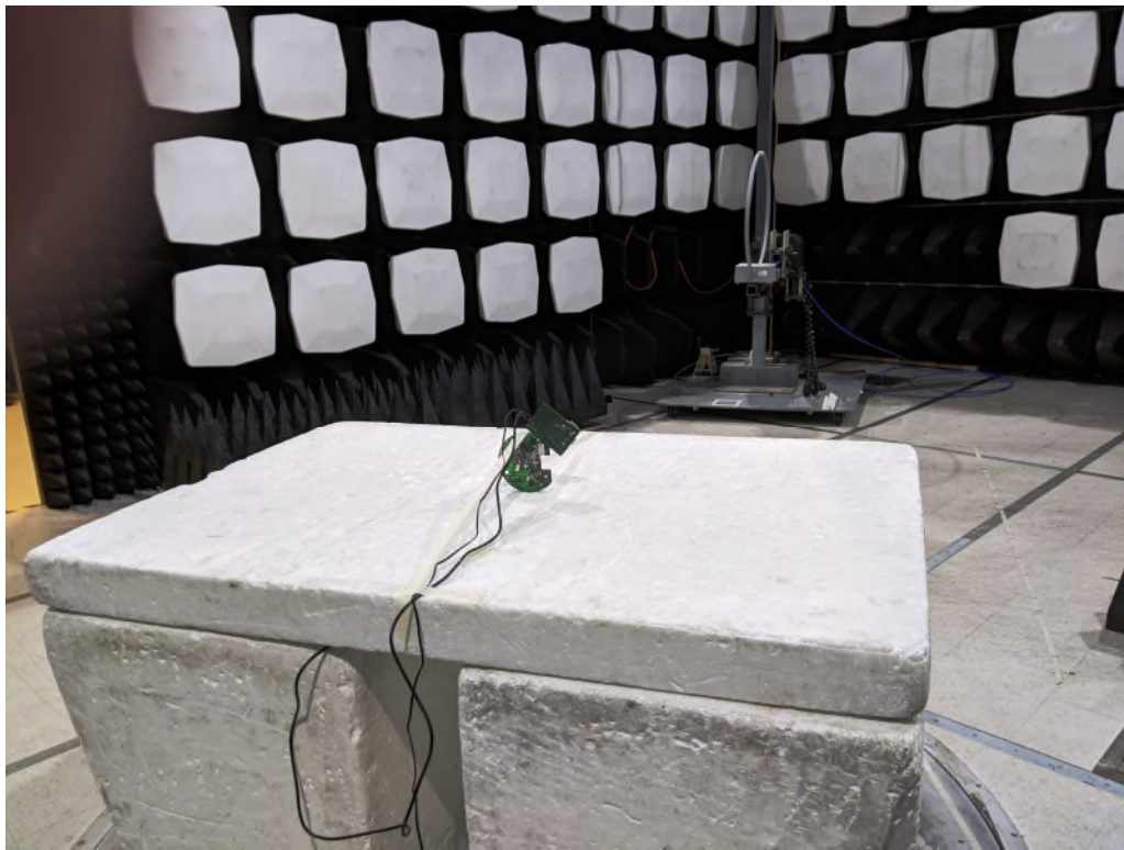
Figure 3: Equipment Under Test – Radiated Emissions <30MHz
