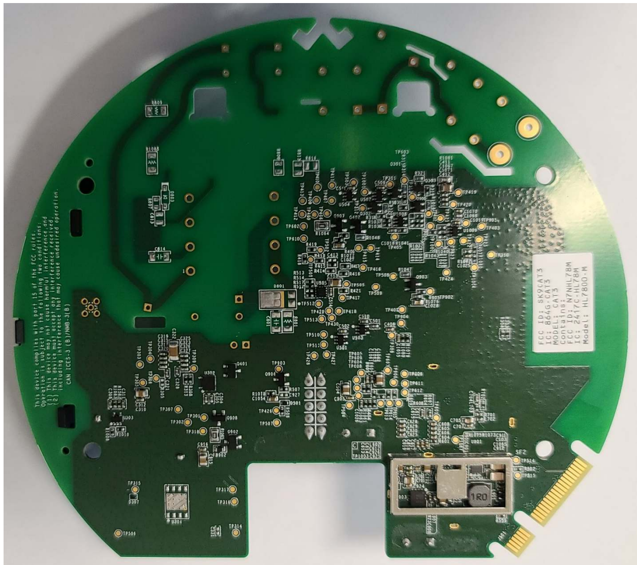
Rear, shields removed
