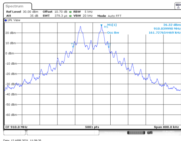
Figure 7.4.1.2-2: 99% Occupied Bandwidth – LCH
