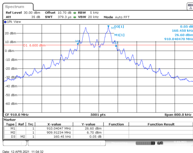
Figure 7.4.1.2-1: 20dB Bandwidth – LCH
