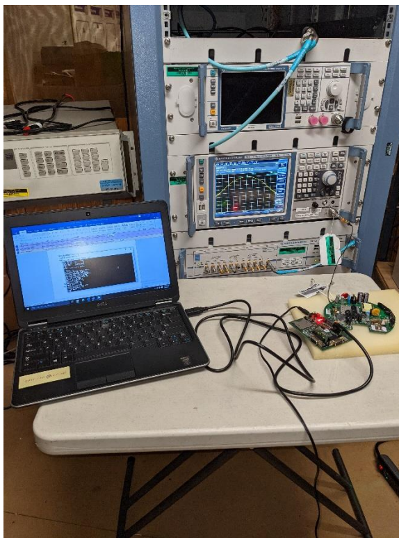
Figure 1: Equipment Under Test – Antenna Port Conducted Measurements
