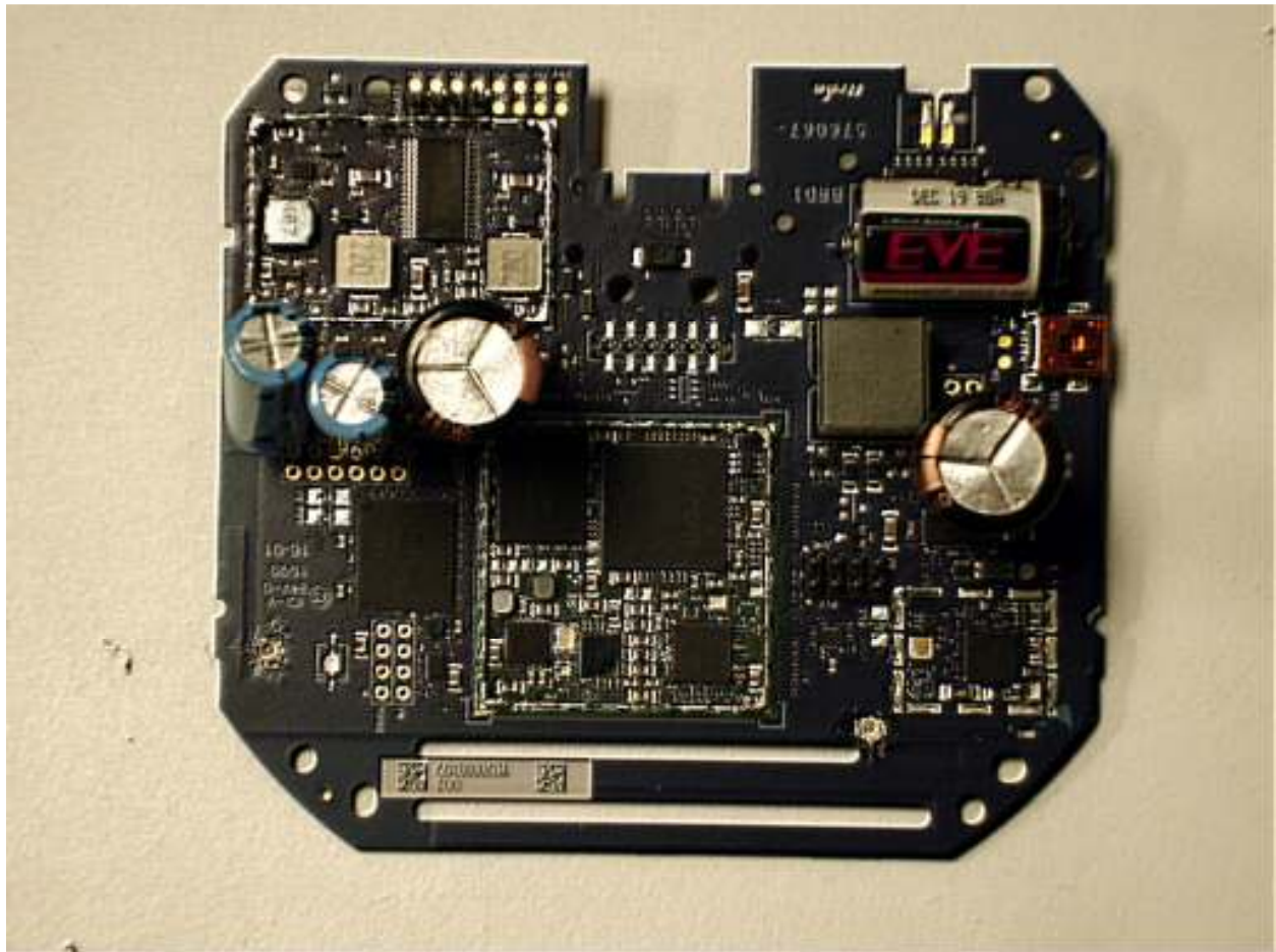
Rear, shields removed
