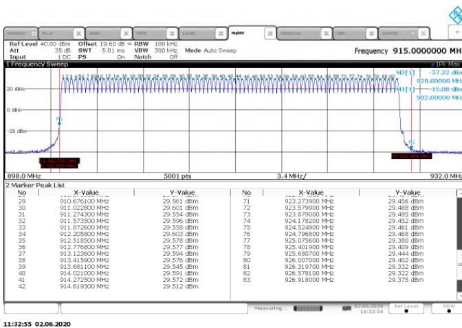
Figure 7.4.2.2-3: No. of Channels – GFSK – 150kbps
