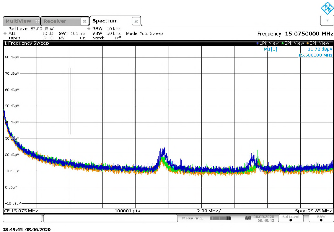
Figure A-2: Radiated Spurious Emissions – 150 kHz to 30 MHz
