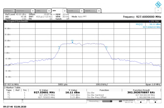
Figure 7.4.4.2-12: Sample Plot 99% OBW - OFDM - 600kbps
