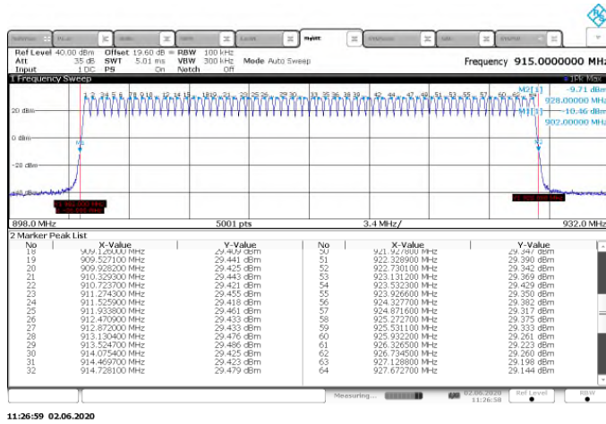
Figure 7.4.2.2-5: No. of Channels – GFSK – 300kbps
