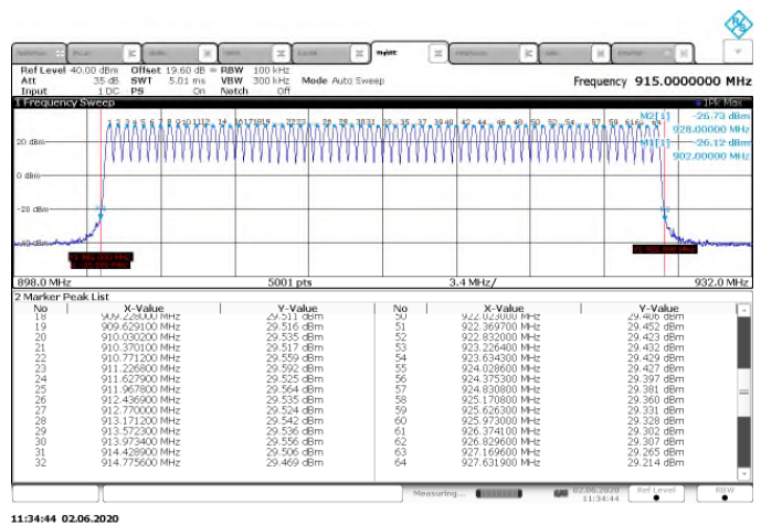
Figure 7.4.2.2-2: No. of Channels – FSK – 150kbps
