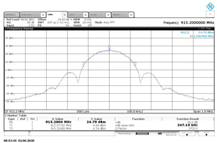
Figure 7.4.4.2-4: Sample Plot 20dB BW - GFSK - 200kbps
