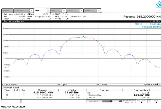
Figure 7.4.4.2-1: Sample Plot 20dB BW - FSK - 100kbps
