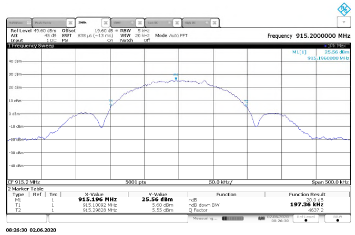
Figure 7.4.4.2-2: Sample Plot 20dB BW - FSK - 150kbps
