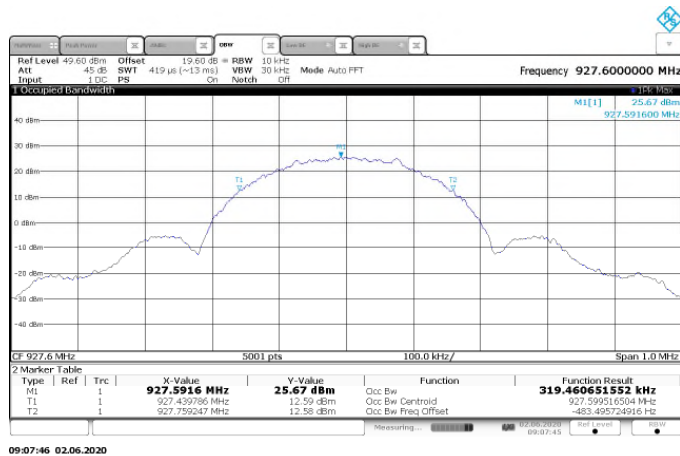
Figure 7.4.4.2-11: Sample Plot 99% OBW - GFSK - 300kbps
