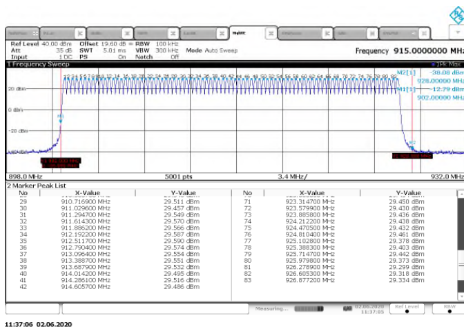
Figure 7.4.2.2-1: No. of Channels – FSK – 100kbps
