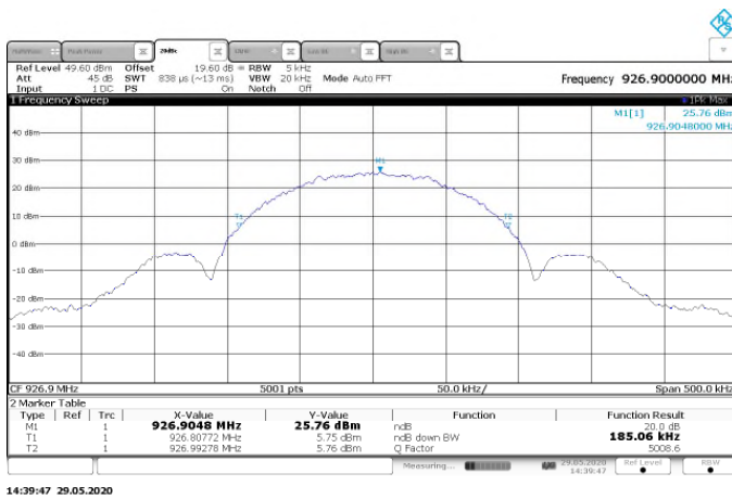
Figure 7.4.4.2-3: Sample Plot 20dB BW - GFSK - 150kbps
