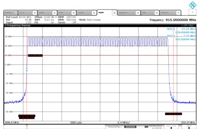
Figure 7.5.1.2-16: Band Edges – GFSK – 200kbps
