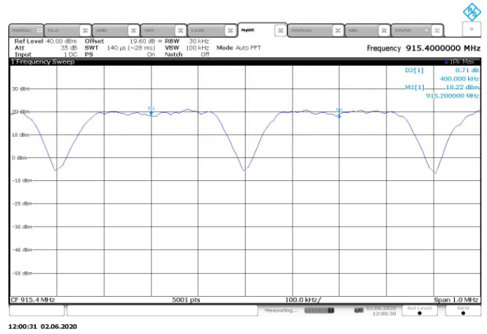
Figure 7.4.1.2-6: Freq. Separation – OFDM – 600kbps
