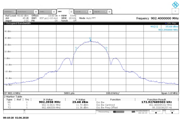
Figure 7.4.4.2-8: Sample Plot 99% OBW - FSK - 150kbps
