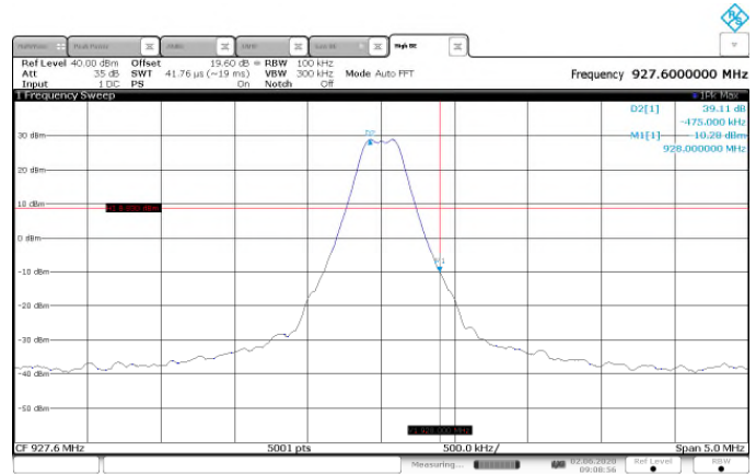
Figure 7.5.1.2-10: Upper Band-edge – GFSK – 300kbps
