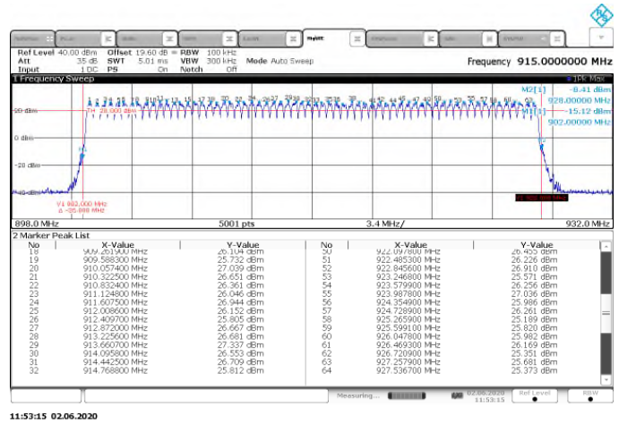
Figure 7.4.2.2-6: No. of Channels – OFDM – 600kbps
