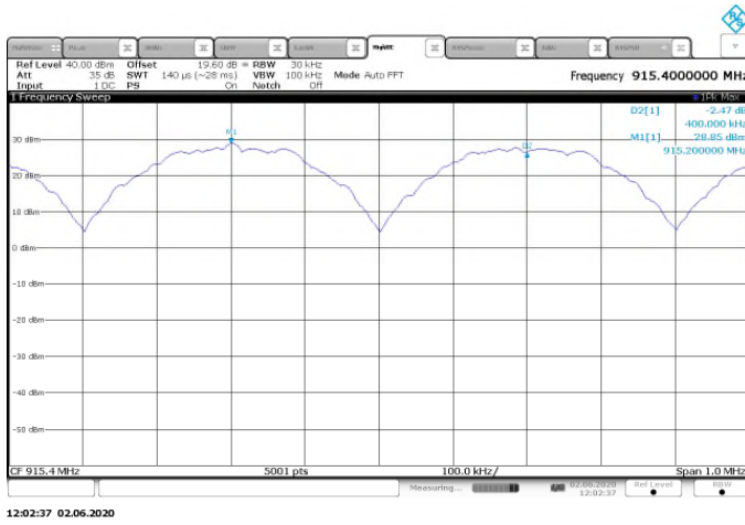
Figure 7.4.1.2-5: Freq. Separation – GFSK – 300kbps
