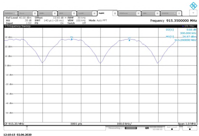
Figure 7.4.1.2-4: Freq. Separation – GFSK – 200kbps
