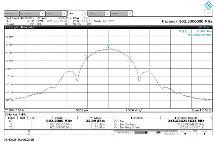
Figure 7.4.4.2-10: Sample Plot 99% OBW - GFSK - 200kbps
