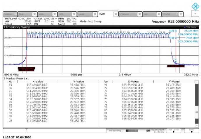
Figure 7.4.2.2-4: No. of Channels – GFSK – 200kbps
