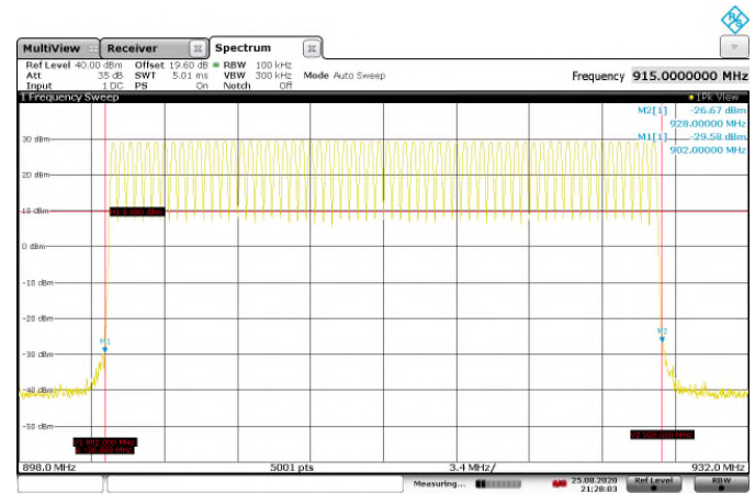
Figure 7.5.1.2-14: Band Edges – FSK – 150kbps
