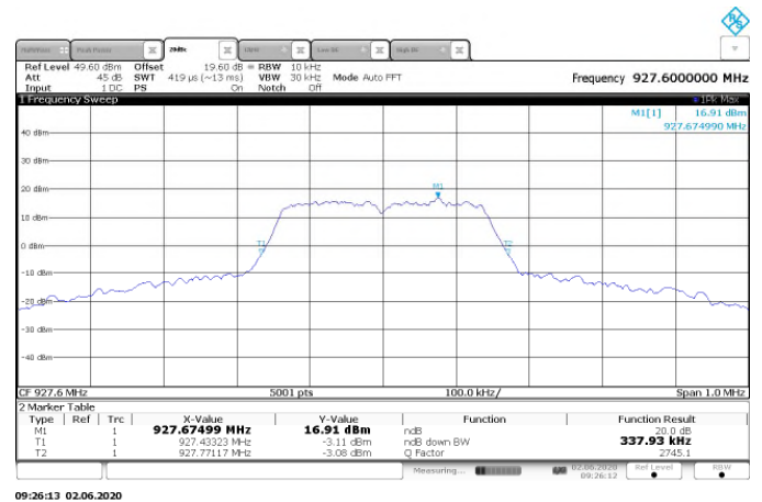
Figure 7.4.4.2-6: Sample Plot 20dB BW - OFDM - 600kbps
