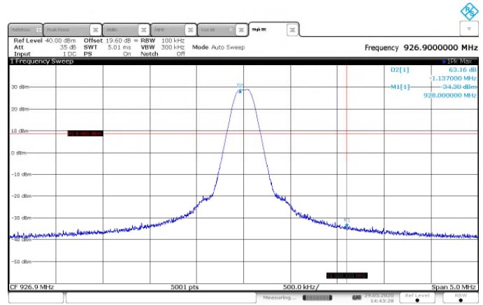
Figure 7.5.1.2-6: Upper Band-edge – GFSK – 150kbps
