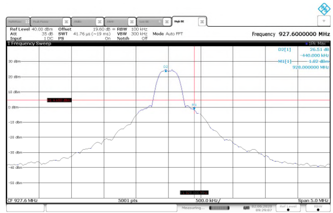
Figure 7.5.1.2-12: Upper Band-edge – OFDM – 600kbps
