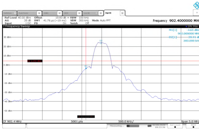
Figure 7.5.1.2-11: Lower Band-edge – OFDM – 600kbps
