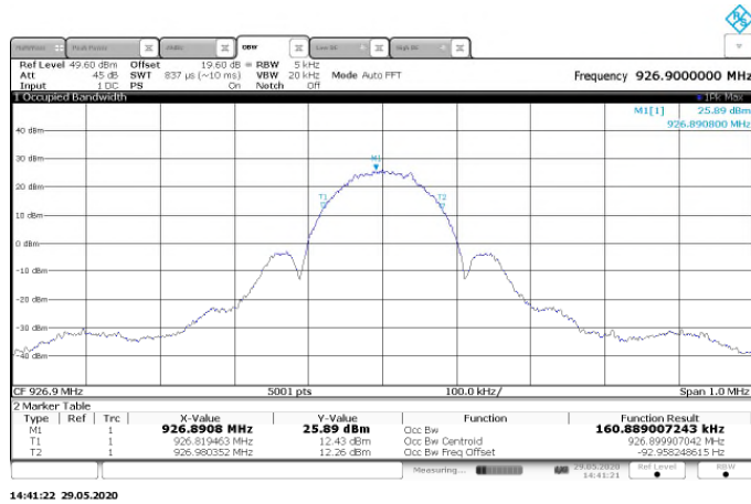
Figure 7.4.4.2-9: Sample Plot 99% OBW - GFSK - 150kbps
