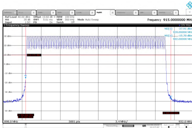
Figure 7.5.1.2-15: Band Edges – GFSK – 150kbps
