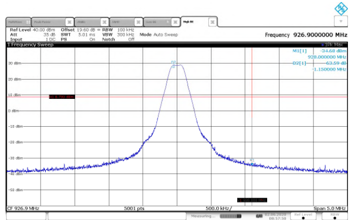
Figure 7.5.1.2-8: Upper Band-edge – GFSK – 200kbps
