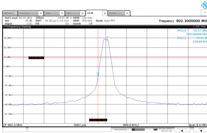
Figure 7.5.1.2-7: Lower Band-edge – GFSK – 200kbps
