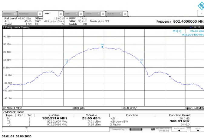
Figure 7.4.4.2-5: Sample Plot 20dB BW - GFSK - 300kbps
