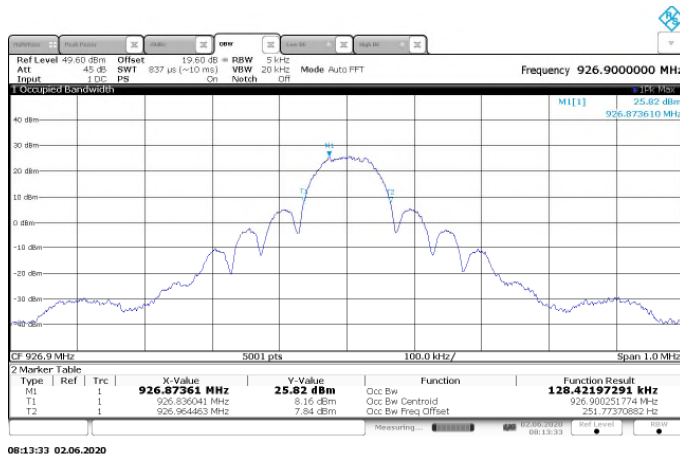
Figure 7.4.4.2-7: Sample Plot 99% OBW - FSK - 100kbps
