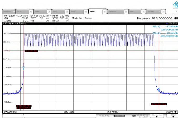
Figure 7.5.1.2-13: Band Edges – FSK – 100kbps
