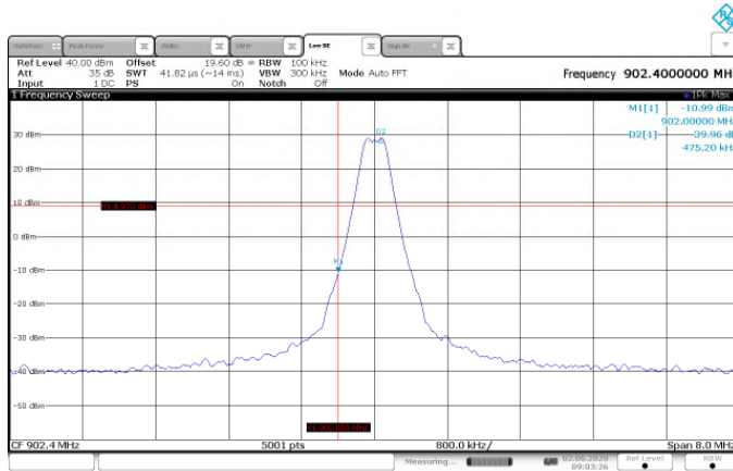
Figure 7.5.1.2-9: Lower Band-edge – GFSK – 300kbps
