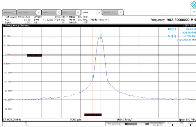
Figure 7.5.1.2-5: Lower Band-edge – GFSK – 150kbps
