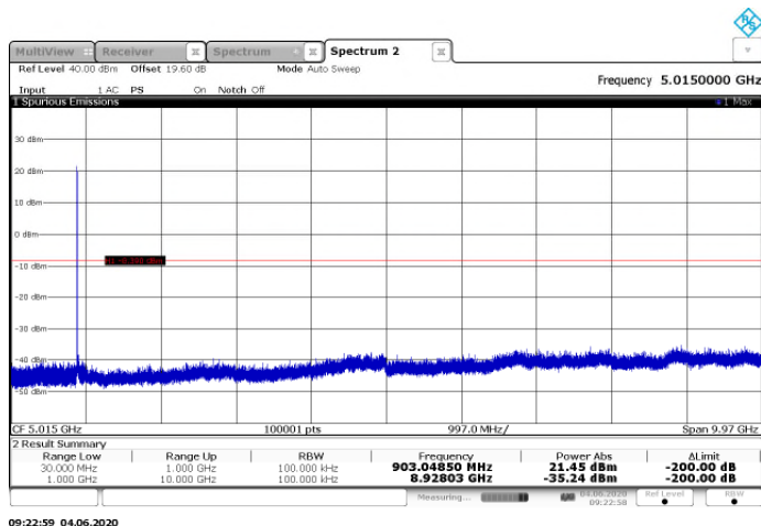
Figure 7.5.1.2-1: 30 MHz – 10 GHz – Low Channel (2400k)
