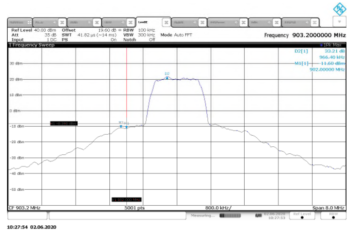
Figure 7.5.1.2-6: Lower Band-edge (2400k)
