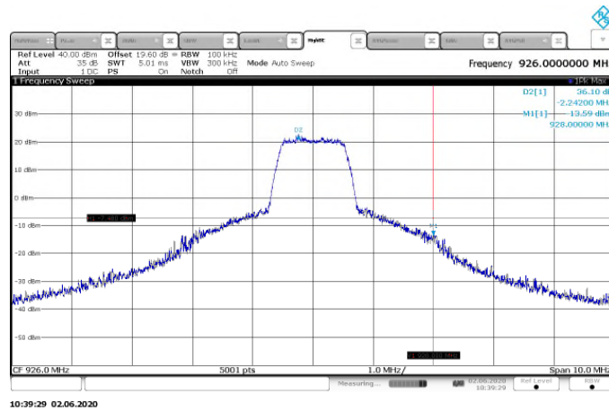
Figure 7.5.1.2-7: Upper Band-edge (2400k)
