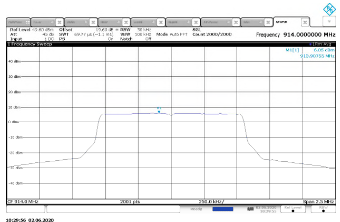
Figure 7.6.2-2: Sample Power Spectral Density – MCH (2400k)
