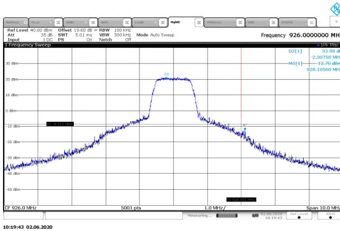
Figure 7.5.1.2-5: Upper Band-edge (1200k)
