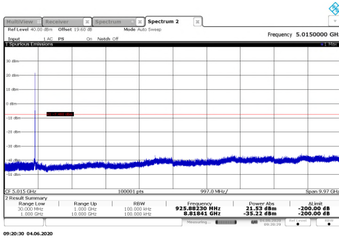
Figure 7.5.1.2-3: 30 MHz – 10 GHz –High Channel (2400k)
