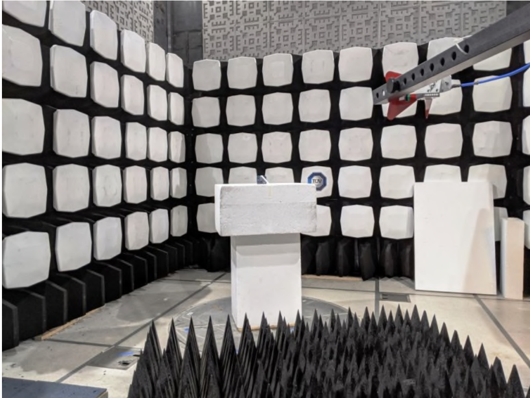
Figure 7: Test Setup – Radiated Emissions >1GHz
