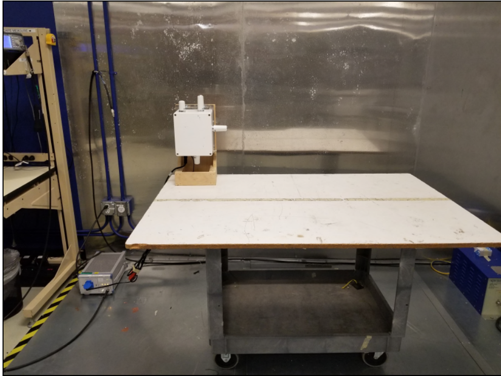
Figure 9: Equipment Under Test – AC Conducted Emissions
