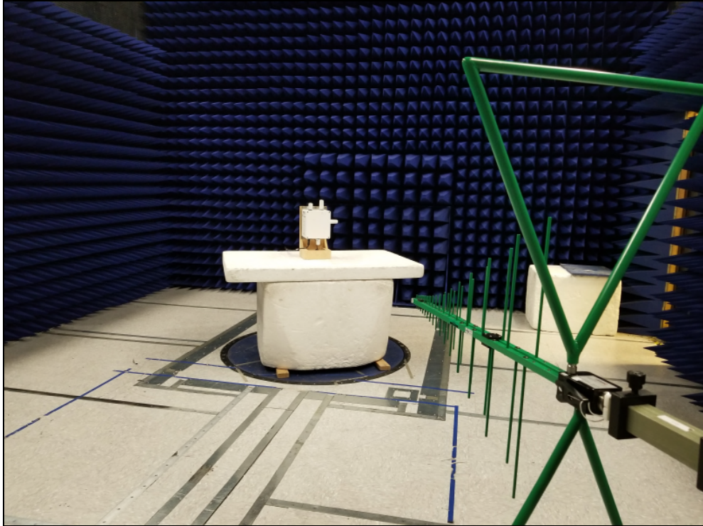
Figure 2: Equipment Under Test – Radiated Emissions <1GHz
