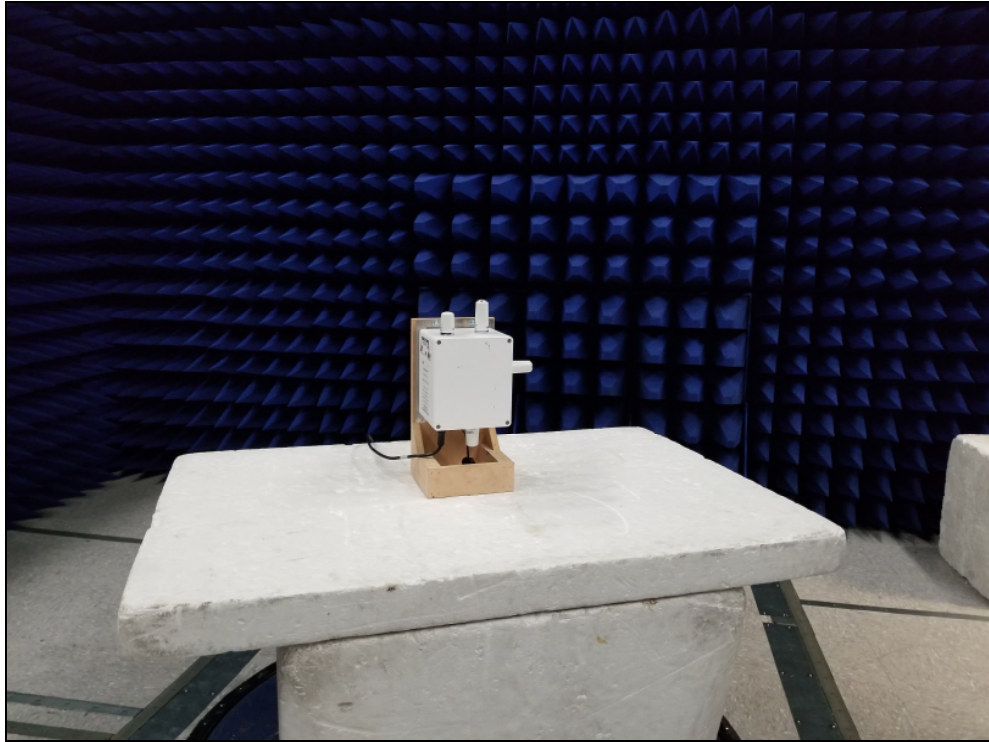
Figure 1: Equipment Under Test – Radiated Emissions <1GHz
