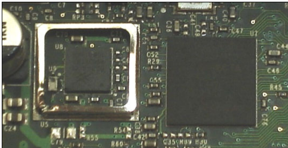
Figure 9: Internal Photo – Zigbee RF Section Shields Removed
