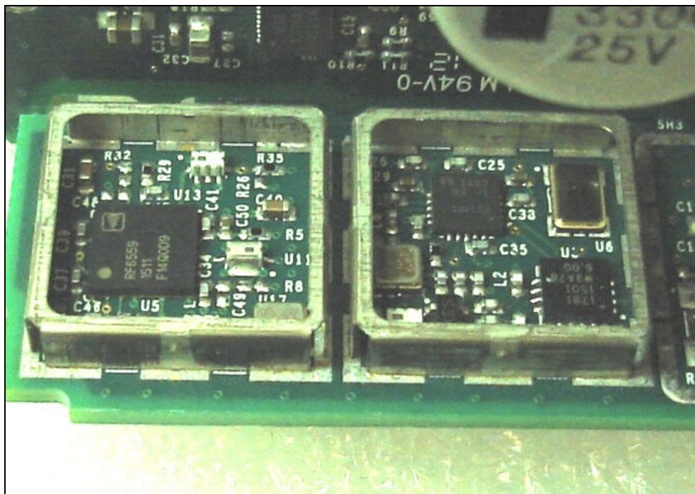
Figure 8: Internal Photo – 900 MHz LAN RF Section Shields Removed
