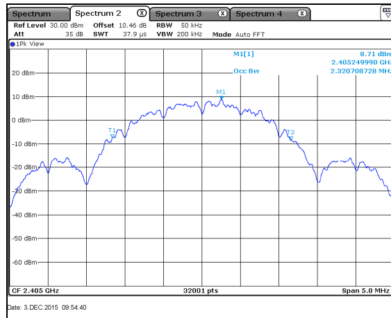
Figure 7.3.2-4: 99% Bandwidth Plot – CH 11
