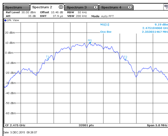
Figure 7.3.2-6: 99% Bandwidth Plot – CH 25
