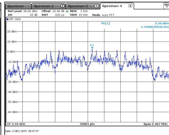
Figure 7.6.2-2: PSD Plot – CH18
