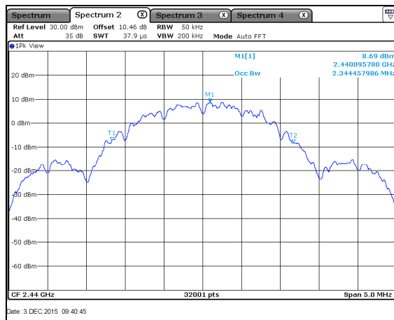
Figure 7.3.2-5: 99% Bandwidth Plot – CH 18
