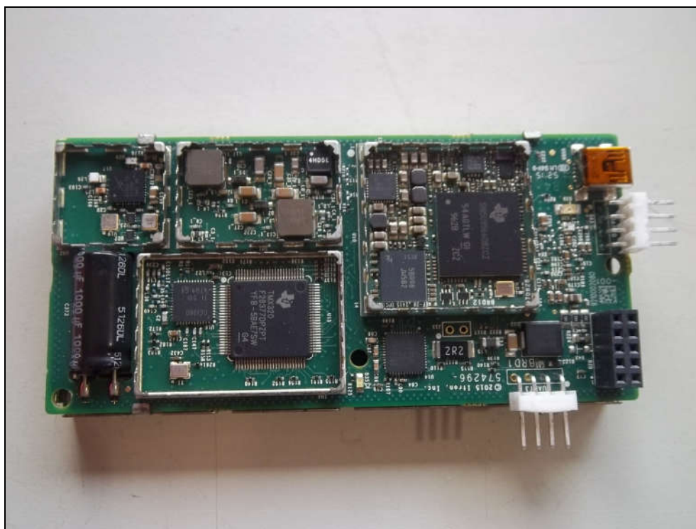
Figure 2: External/Internal Photo – Shields Removed
