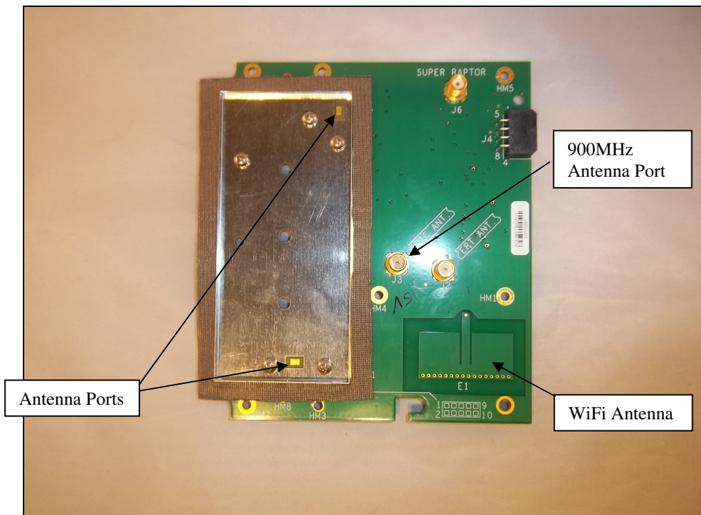
Figure 4: Internal Photo
