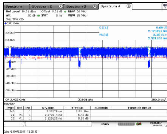
Figure 7.7.2-4: Duty Cycle 802.11n (HT 40)
