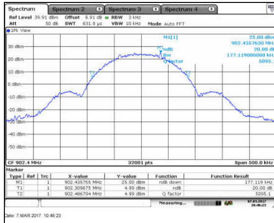
Figure 7.4.4.2-7: 20dB BW Low Ch - FSK - 150kbps
