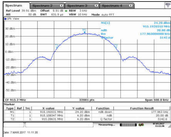
Figure 7.4.4.2-8: 20dB BW Mid Ch - FSK - 150kbps
