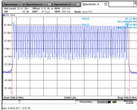
Figure 7.4.2.2-1: No. of Hopping Ch – FSK – 50kbps
