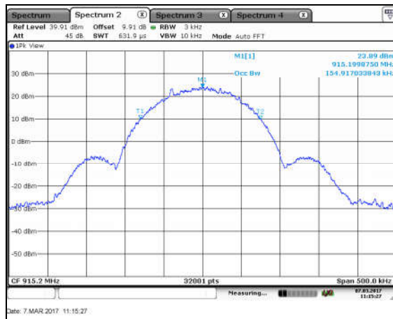
Figure 7.4.4.2-11: 99% BW Mid Ch - FSK - 150kbps
