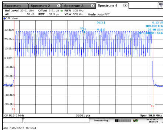
Figure 7.4.2.2-2: No. of Hopping Ch – FSK – 150kbps
