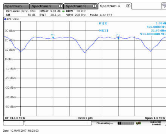
Figure 7.4.1.2-4: Freq. Separation – OFDM – 600kbps
