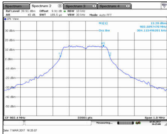
Figure 7.4.4.2-16: 99% BW Low Ch – OFDM – 200kbps
