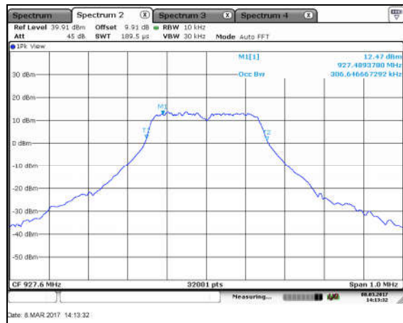
Figure 7.4.4.2-18: 99% BW High Ch – OFDM – 200kbps
