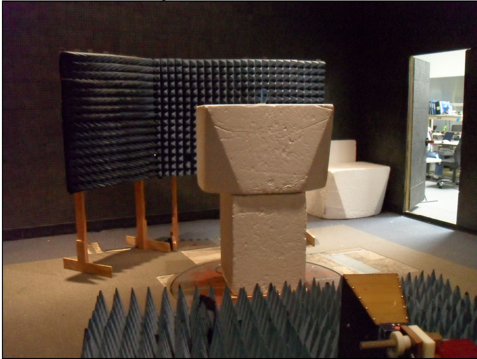
Figure 1: Radiated Emissions
