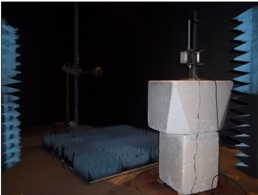
Figure 2: Radiated Emissions
