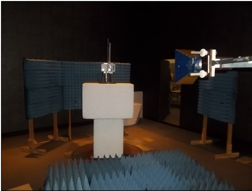
Figure 1: Radiated Emissions
