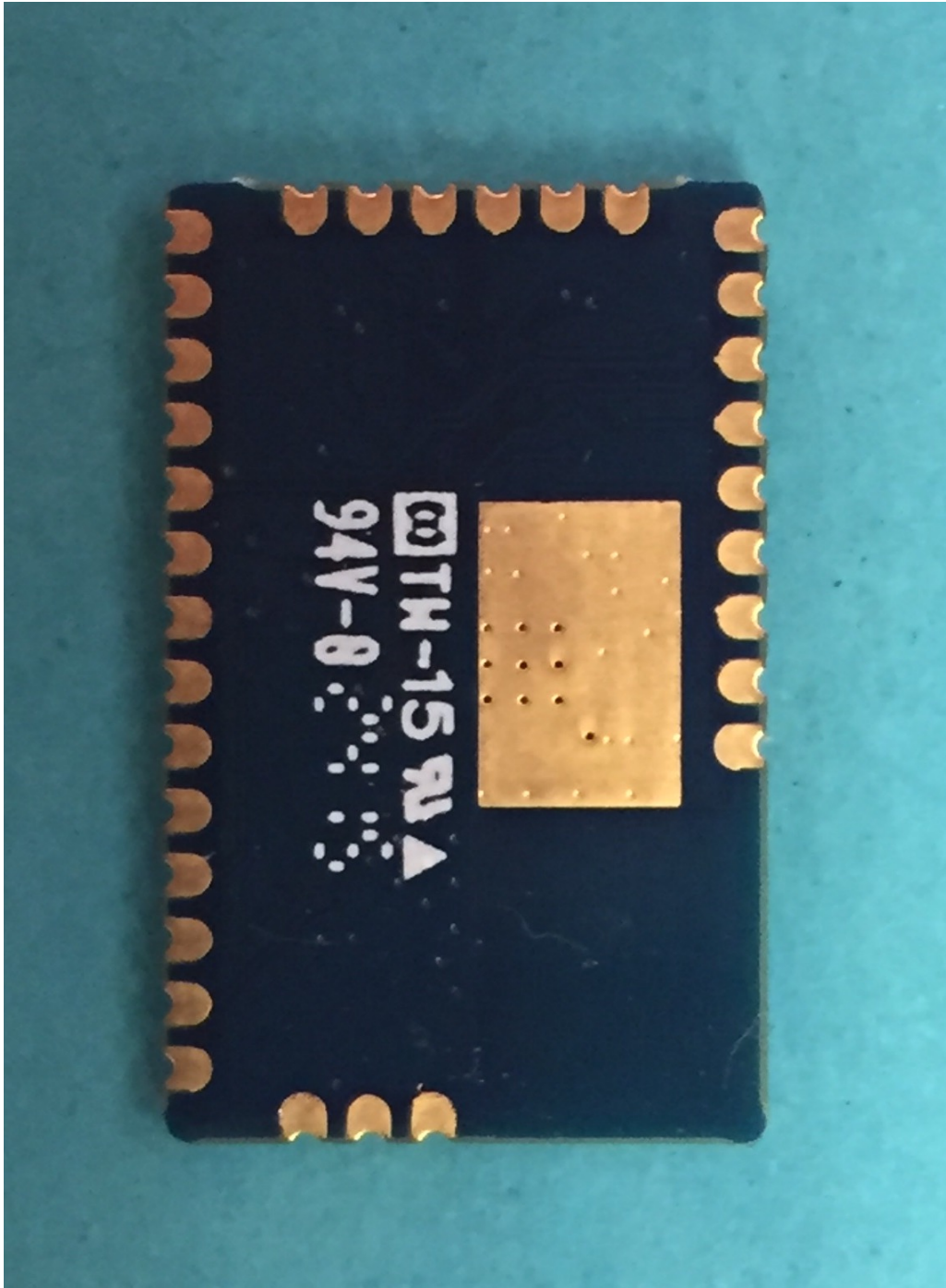
PCB Bottom View
