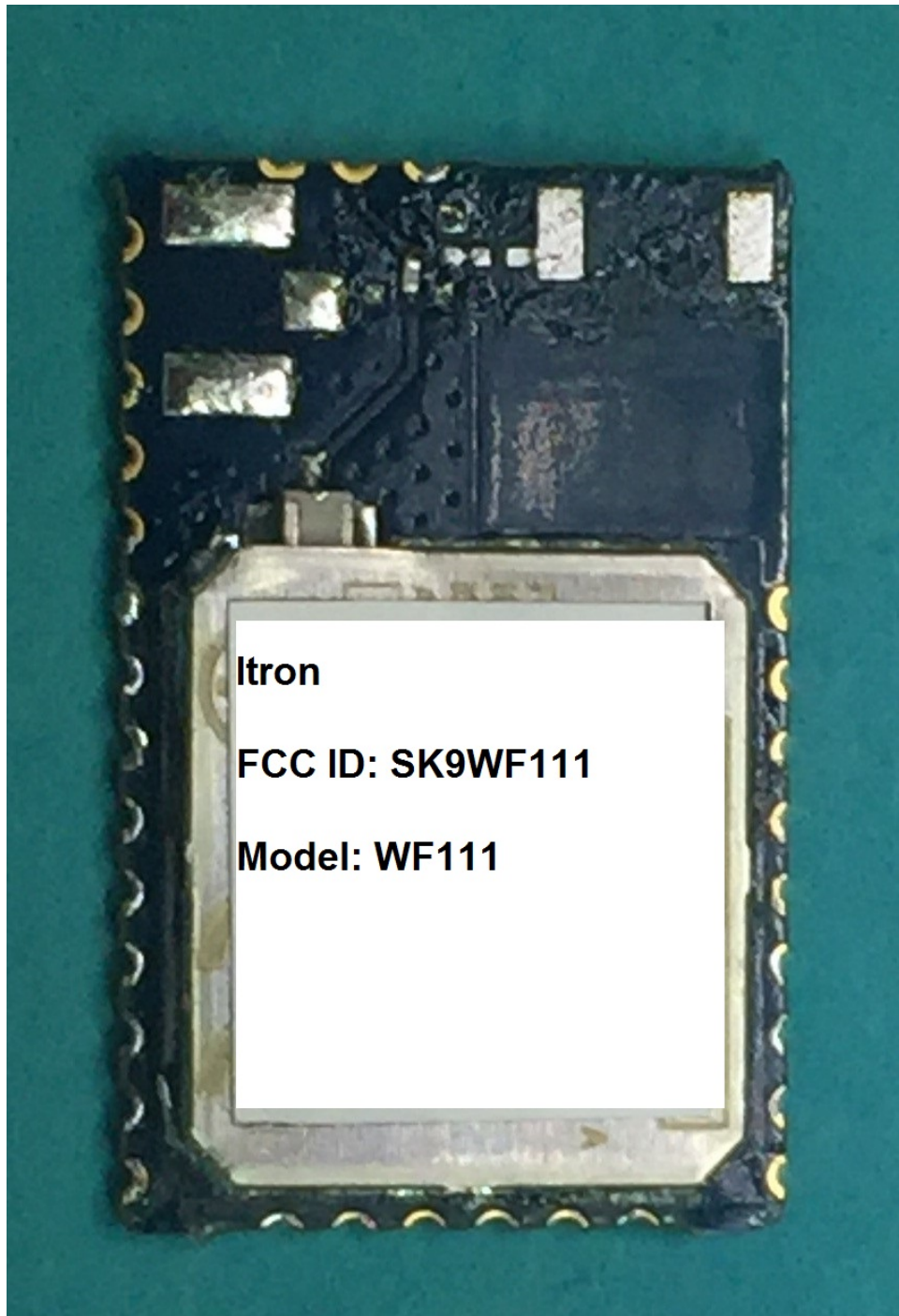
PCB Top View with Shields
