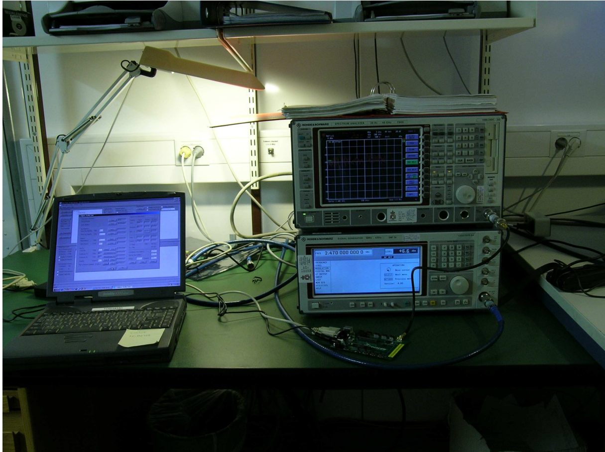
13213-SRB - Test set-up for Conducted measurements
