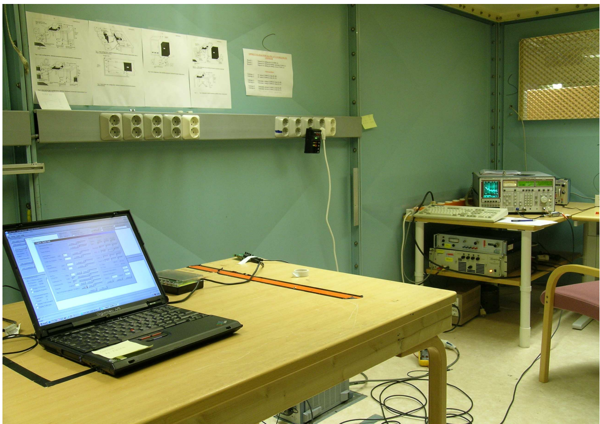
13213-SRB – Conducted emission test set-up
