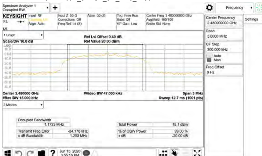
OBW 20dB_8DPSK_3M_DH5_2480MHz
