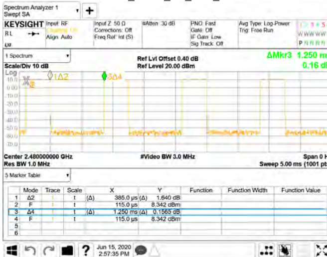
Dwell Time_GFSK_1M_DH1_2480MHz
