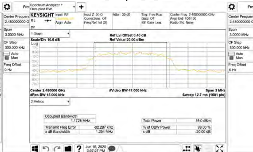
OBW 20dB_π/4DQPSK_2M_2480MHz
