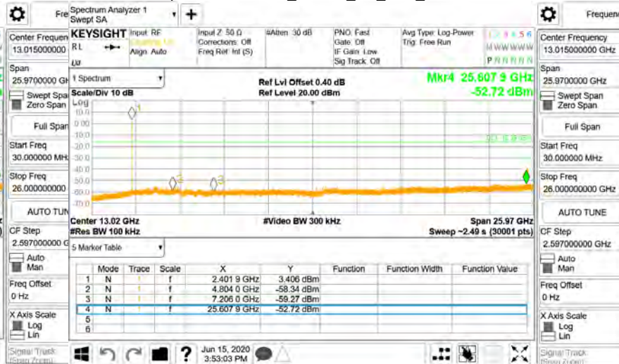
Spurious Emission_8DPSK_3M_DH5_2402MHz
