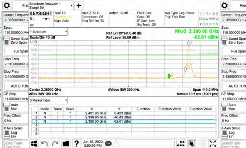
Band Edge_8DPSK_3M_DH5_2402MHz
