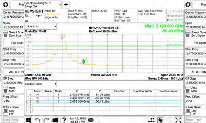
Band Edge_8DPSK_3M_DH5_2480MHz
