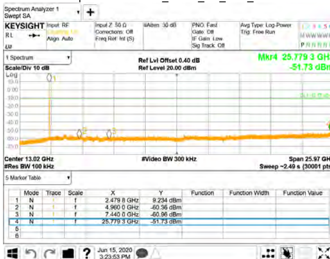
Spurious Emission_GFSK_1M_DH5_2480MHz
