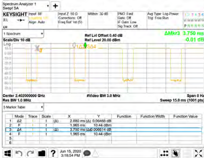
Dwell Time_GFSK_1M_DH5_2402MHz
