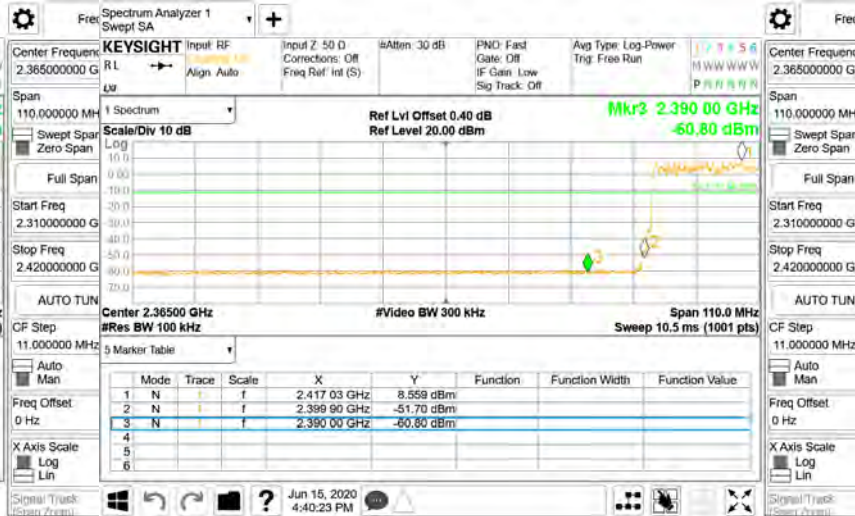
Hopping Band Edge_8DPSK_3M_DH5_2402MHz
