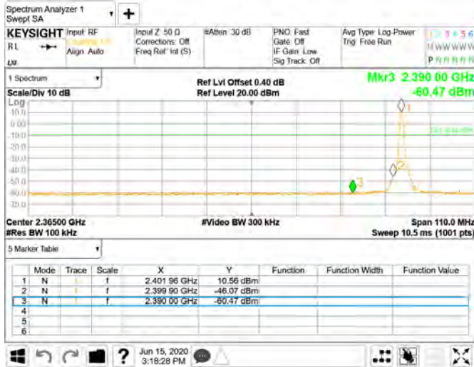
Band Edge_GFSK_1M_DH5_2402MHz
