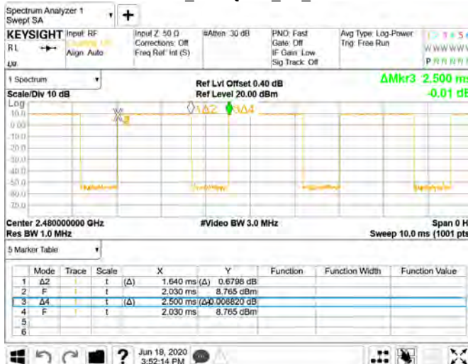
Dwell Time \pi/4 DQPSK_2M_2480MHz
