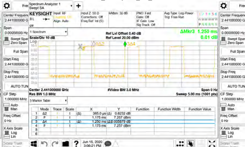
Dwell Time_π/4QPSK_2M_2441MHz
