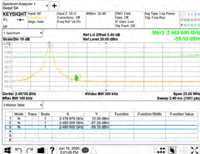
Band Edge_GFSK_1M_DH5_2480MHz
