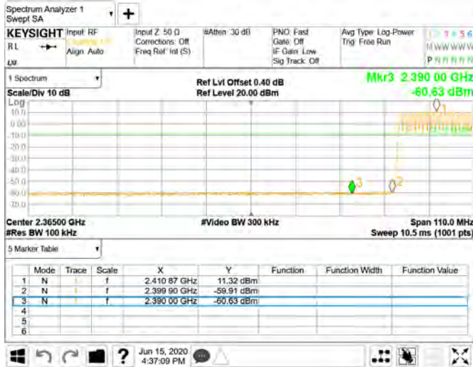
Hopping Band Edge_GFSK_1M_DH5_2402MHz
