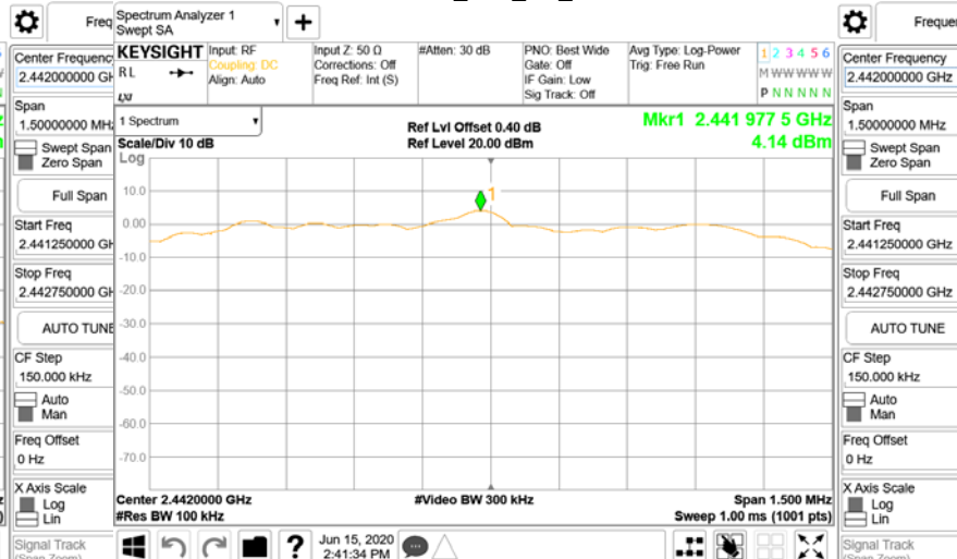
Reference Level_BLE_2M_MidCH20-2442
