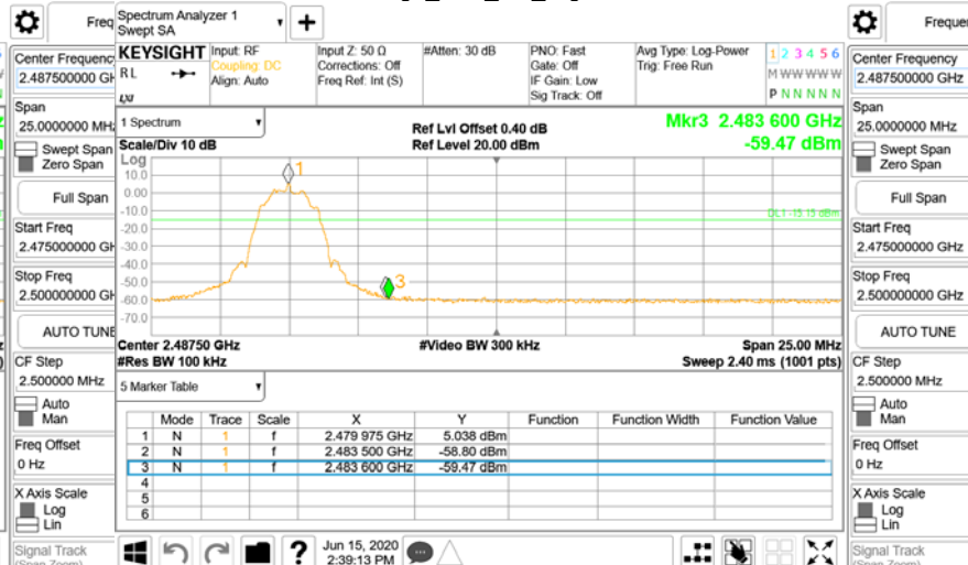
Band Edge_BLE_2M_HighCH39-2480
