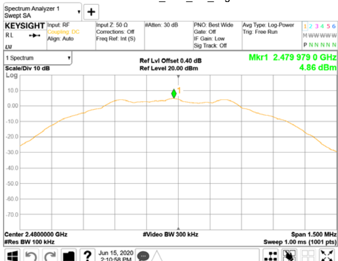
Reference Level_BLE_1M_HighCH39-2480
