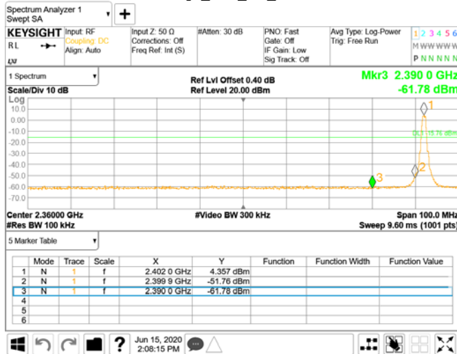
Band Edge_BLE_1M_LowCH00-2402
