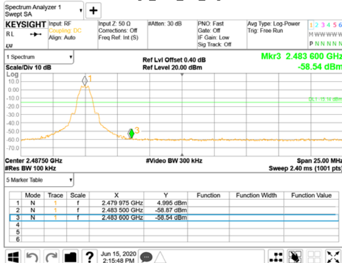
Band Edge_BLE_1M_HighCH39-2480
