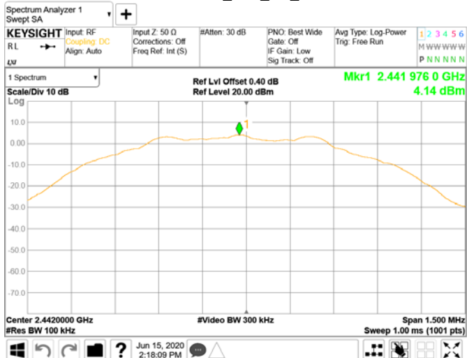
Reference Level_BLE_1M_MidCH20-2442
