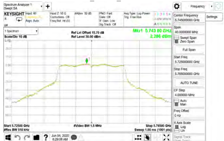
802.11a_20MHz_5745MHz
