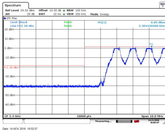
Figure 8.4-6: Conducted spurious emissions at the lower band edge hopping, Modulation 1
