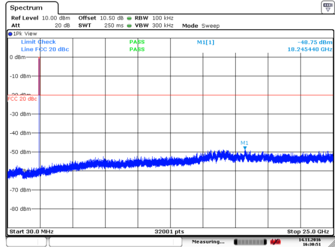
Figure 8.4-2: Conducted spurious emissions for mid channel, Modulation 1
