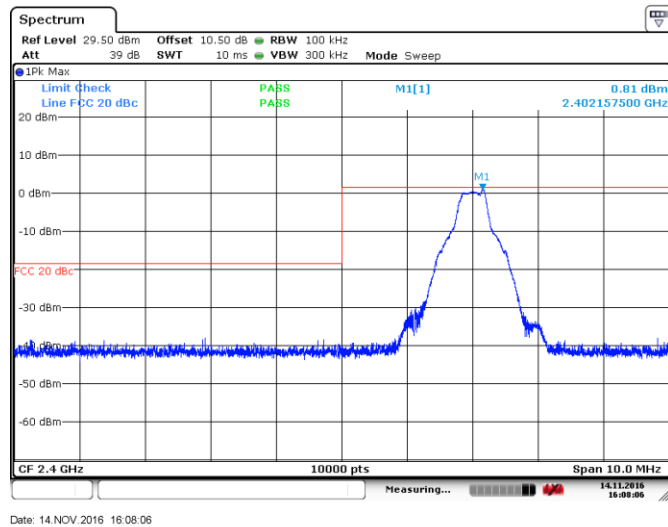
Figure 8.4-4: Conducted spurious emissions at the lower band edge, Modulation 1
