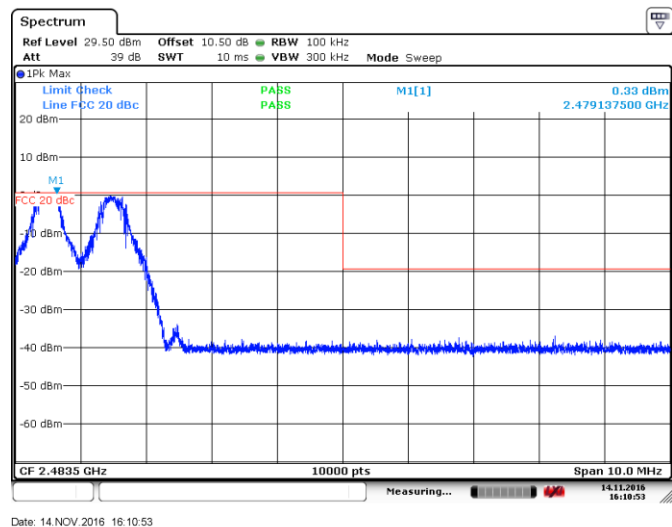
Figure 8.4-7: Conducted spurious emissions for high channel hopping, Modulation 1
