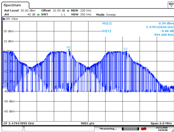
Figure 8.2-4: Carrier frequency separation Modulation 1
