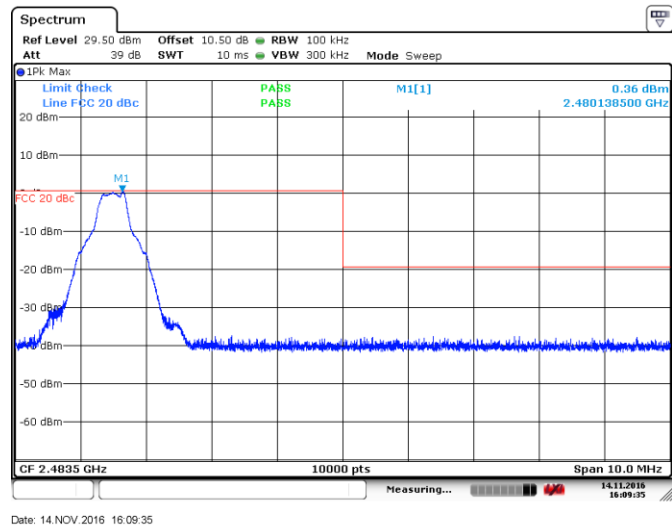
Figure 8.4-5: Conducted spurious emissions at the upper band edge, Modulation 1
