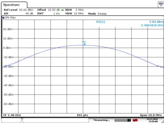
Figure 8.3-6: Output power on high channel, Modulation 2
