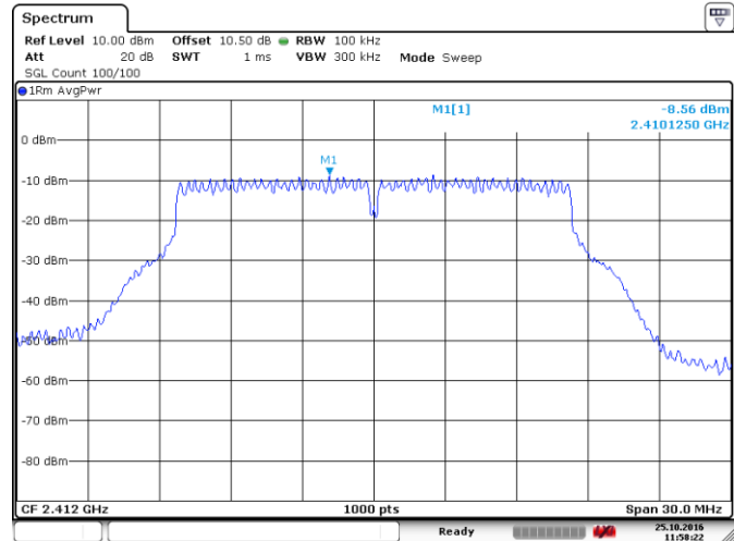
Figure 8.5-2: PSD sample plot on 802.11g
