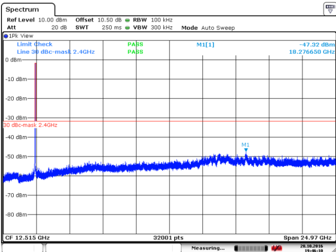
Figure 8.4-3: Conducted spurious emissions for 802.11n HT20 (TX 2412 MHz)
