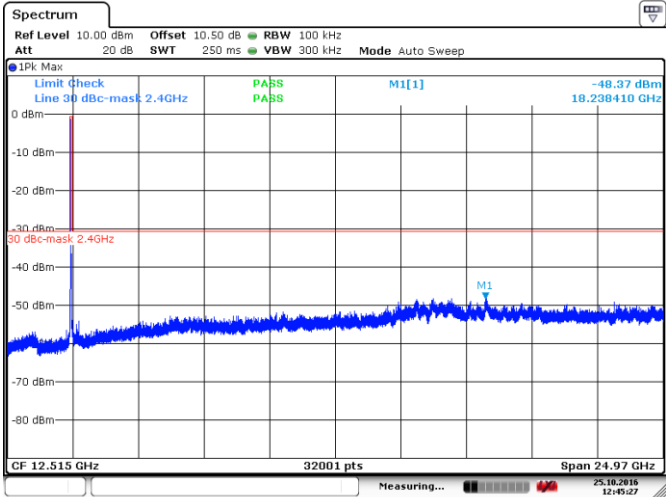
Figure 8.4-5: Conducted spurious emissions for 802.11g (TX 2437 MHz)
