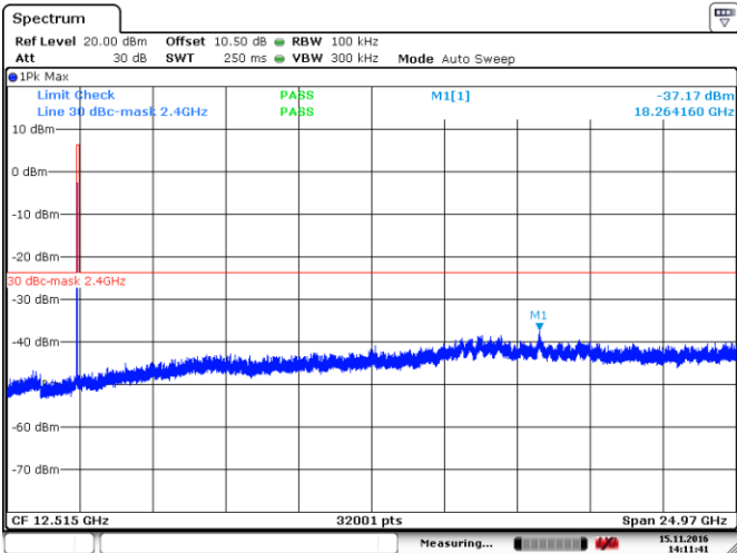
Figure 8.4-1: Conducted spurious emissions for 802.11b (TX 2412 MHz)
