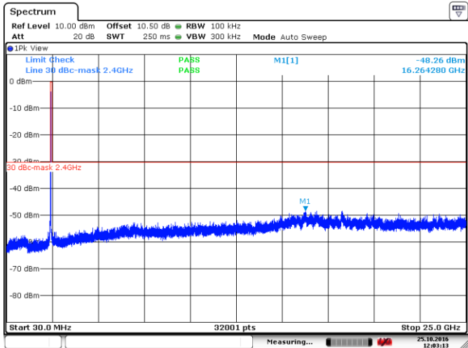
Figure 8.4-2: Conducted spurious emissions for 802.11g (TX 2412 MHz)
