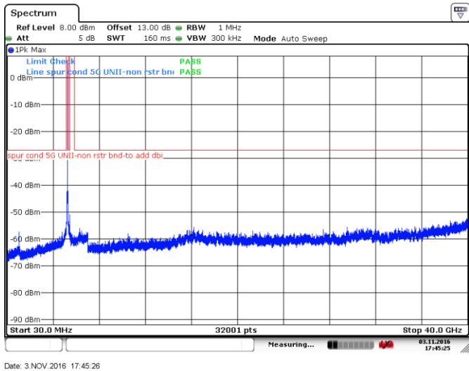
Figure 8.4-17: Conducted peak spurious emissions outside restricted bands at high channel, 802.11a
