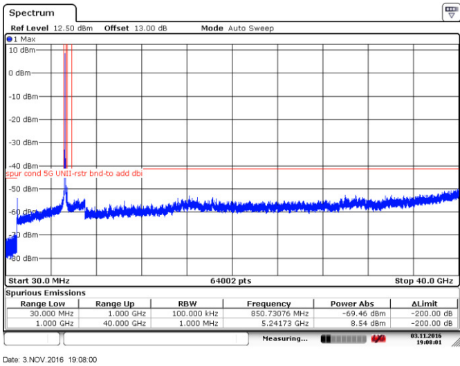
Figure 8.4-11: Conducted peak spurious emissions within restricted bands at high channel, 802.11ac-VHT20
