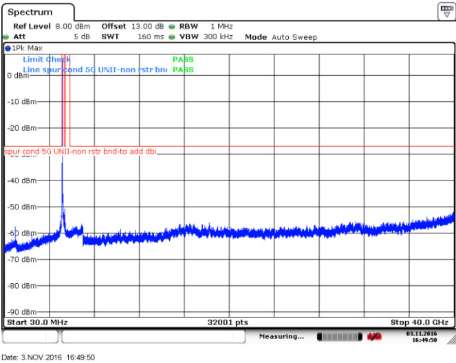
Figure 8.4-15: Conducted peak spurious emissions outside restricted bands at low channel, 802.11a
