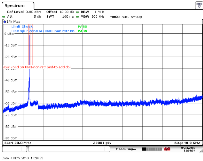
Figure 8.4-28: Conducted peak spurious emissions outside restricted bands, 802.11ac-VHT80
