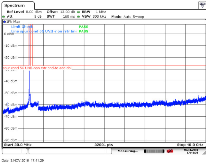
Figure 8.4-16: Conducted peak spurious emissions outside restricted bands at mid channel, 802.11a
