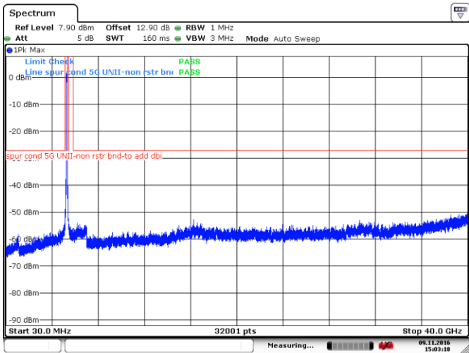
Figure 8.4-28: Peak spurious emissions outside restricted bands, 802.11ac-VHT80, ch52
