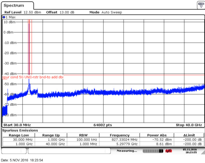
Figure 8.4-5: Peak spurious emissions within restricted bands at mid channel, 802.11n-HT20, ch60
