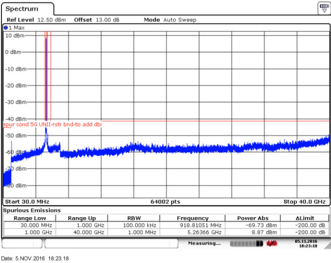
Figure 8.4-4: Peak spurious emissions within restricted bands at low channel, 802.11n-HT20, ch52
